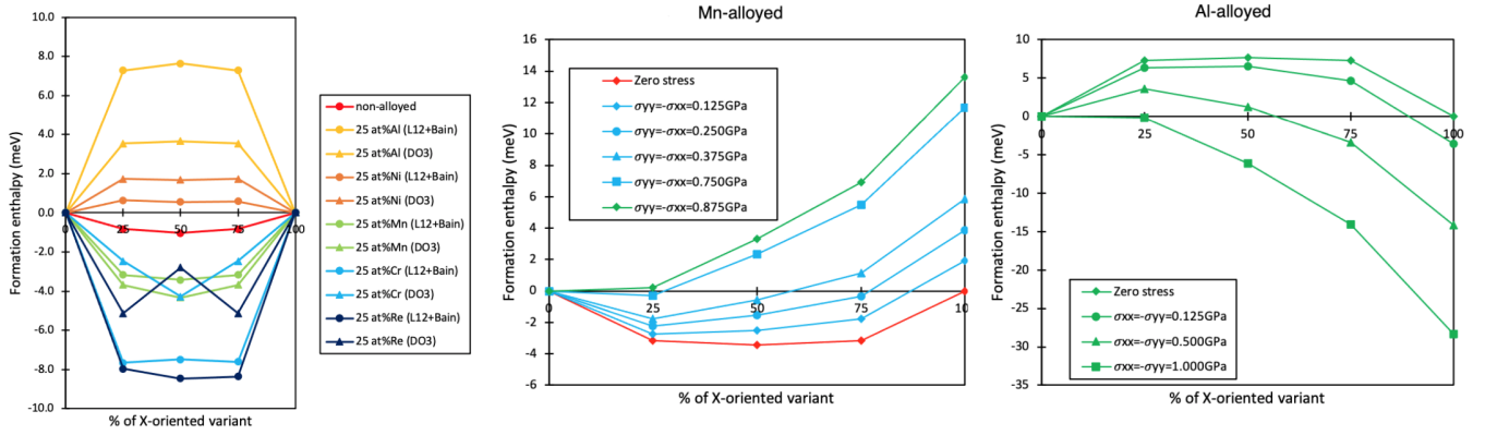
Figure 3: Crystal twin formation enthalpy for alloyed martensite (reference: 0%X variant taken under same stress). Left: under zero stress. Center (resp. right): case of Mn-alloyed (resp. Al-alloyed) martensite, under imposed shear stress.
