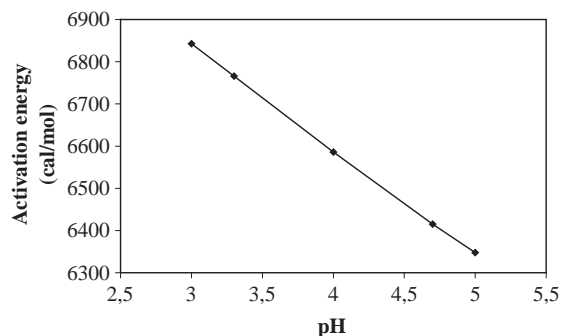
Fig. 3. Influence of pH on the activation energy for S. bayanus var. uvarum growth (derived from log \mu as a function of 1/ T ).
