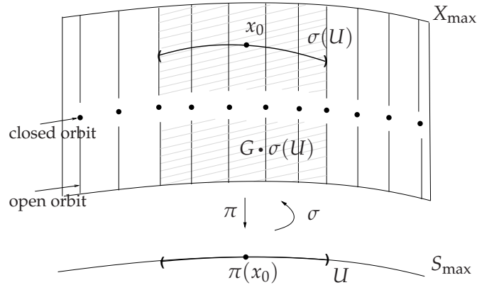
FIGURE 1. The local geometry of the quotient map
