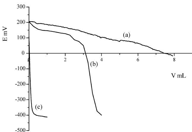
Fig. 1. Evolution of zero current potential of the platinum electrode during introduction of a Ti(III) solution in various oxygen concentrations. Model wine solution volume: 20 \text{ mL} . Ti(III) concentration: 4.8 \times 10^{-3} \text{ mol L}^{-1} . (a) Volume increment 30 \mu\text{L} , strongly stirred solution. (b) Volume increment: 250 \mu\text{L} , gently stirred solution. (c) Initially deaerated solution and N_2 bubbling during Ti(III) introduction.
