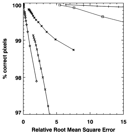
Fig. 12. RRMSE (4) versus SAM classification. RRMSE overreacts to the presence of white noise. White noise (+), spectral smoothing (*), spatial smoothing (x), Gibbs effect ( \diamond ), and JPEG2000 compression ( \square ).
