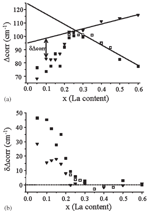
Fig. 5. (a) Variations of \Delta_{\text{corr}} values calculated in the region around the peak at \sim 600\text{cm}^{-1} (squares) and in the full far-IR measured area (down triangles). The open squares and straight lines are as defined for Fig. 3. (b) Excess line width parameter variations against x .
