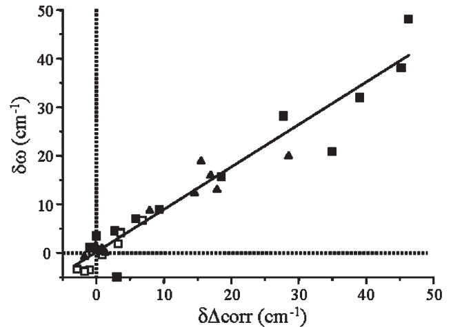
Fig. 6. Change in wavenumber for peaks around 600 and 140\text{cm}^{-1} versus the excess line width parameters extracted from the mid- and far-IR region measurements. Symbols are as defined in Fig. 3.
