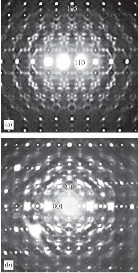
Fig. 11. (a) [\bar{5}11] zone axis EDP of the x = 0.5 cubic sample and (b) \sim[\bar{1}20] zone axis EDP of the x = 0.4 cubic specimen. Note the highly structured complex diffuse intensity distribution accompanying the strong Bragg reflections of the underlying “defect perovskite” cubic average structure.
