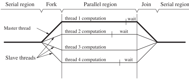
Fig. 3. Fork-join parallelism.
