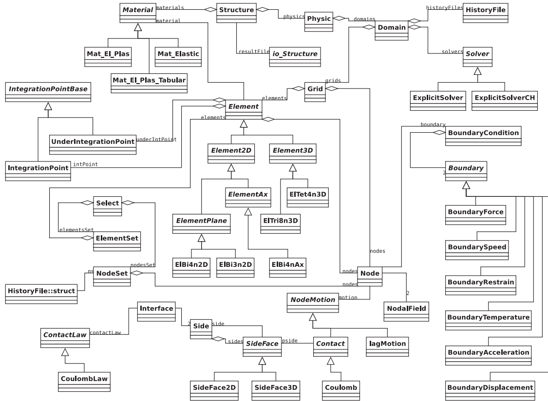
Fig. 2. Simplified UML diagram of the Object oriented framework.
