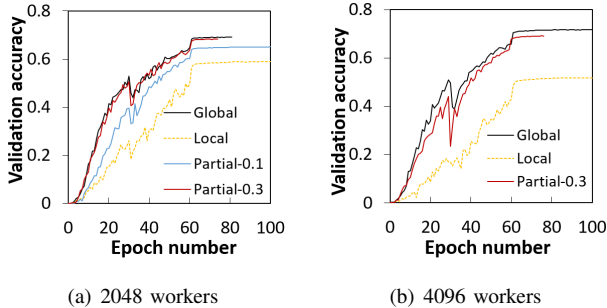
Fig. 6: Top-1 accuracy of ResNet50 with ImageNet-1K on Fugaku when strong scaling (global batch size = 65,536).
