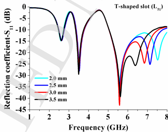
Fig. 8. Reflection coefficient ( S_{11} ) with respect to frequency for various values of L_{S1} ; other parameters are the same as listed in Table 1.
