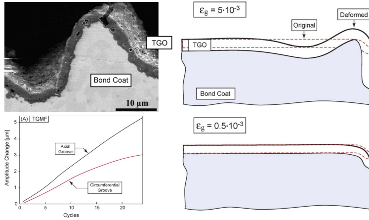
Figure 1.34: Rumppling modeling by initial defect meshing and strain increase associated to oxide growth in plane and out of plane (thickening and lengthening strain) and thermal gradient mechanical fatigue (TGMF) loading [161]
