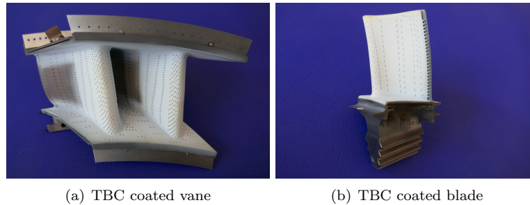
Figure 1.1: TBC coated vane (a) and blade (b) of a GP7000 aero engine
