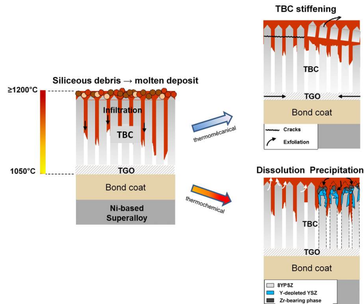
Figure 1.25: CMAS- induced degradation mechanisms of EB-PVD thermal barrier coatings
