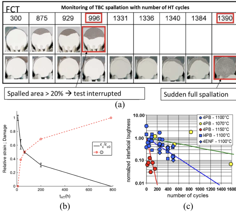
Figure 1.22: Effect of thermal furnace cycling for EB-PVD, (Ni,Pt)Al bond-coat and first generation single crystal superalloy. (a) Appearance of TBC spallation observed on button shape specimens as a function of cycle number, [60], (b) evolution of critical strain, \epsilon_c , at spallation and associated damage, D , as a function of the time spent at high temperature (adapted from [40]), and (c) interfacial toughness as a function of the number of furnace cycles and temperature [195]
