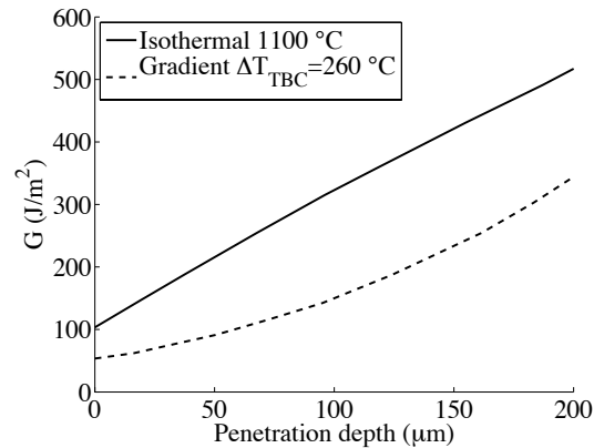
Figure 1.29: Energy release rate ( G ) as a function of CMAS infiltration depth for a delamination crack at the base of a YSZ TBC ( T_{\text{surface}}=1300 \text{ }^\circ\text{C} , T_{\text{bond coat}}=1040 \text{ }^\circ\text{C} and T_{\text{backside}}=800 \text{ }^\circ\text{C} ); comparison with a TBC isothermally heated at 1100 \text{ }^\circ\text{C} (based on information from reference [140])
