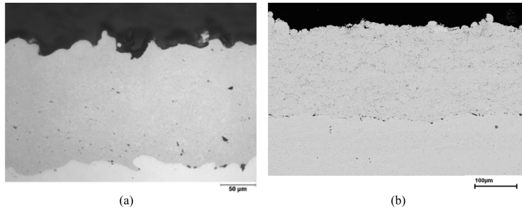
Figure 1.4: SEM micrograph of a VPS (a) and a HVOF bond coat (b).
