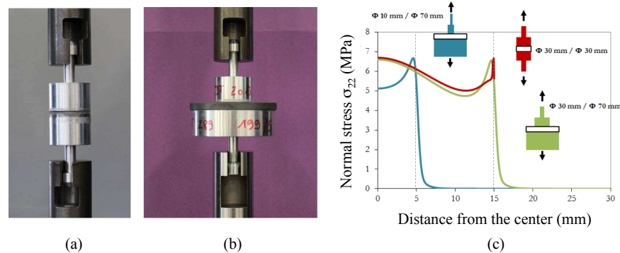
Figure 1.14: Tensile adhesion testing, (a) test configuration with both cylinders glued to the coated sample having the same diameter as the circular sample disc, (b) test configuration with a larger cylinder glued to the substrate side and a smaller to the coating side, with the sample diameter similar to that of the larger cylinder, (c) distribution of the stress component in loading direction from the sample center to the edge for different test configurations (adapted from [141])
