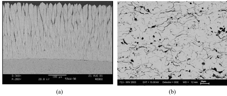
Figure 1.5: SEM micrographs of EB-PVD [64] (a) and APS (b) coatings.
