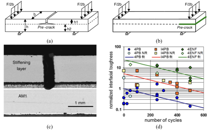
Figure 1.16: Four point bending testing with stiffening layer (a) for mode I testing "4PB" (b) for mode I and mode II "4ENF" (c) detail of notched area for "4PB" test (d) measured interfacial toughness where 4PB corresponds to (a), I4PB same as in (a) except that specimen is upside-down in the set-up so as to promote compression in the top coat and 4ENF corresponds to (b); from [184, 195]
