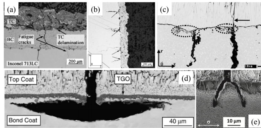
Figure 1.23: Exemplary damages observed under different thermal and mechanical testing conditions, (a) APS BC and TC after LCF test with R_\epsilon=-1 [173], (b) APS BC only, LC after LCF test with R_\epsilon=-1 , and T=850\text{ }^\circ\text{C} [88] (c) EB-PVD TC and APS BC, IP-TMF test: R_\epsilon=0 , \epsilon_a=0.7\% and 100;T;1000\text{ }^\circ\text{C} [190] (d) IP-TGMF test: R_\sigma=0 , \sigma_a=100\text{ MPa} and 100;T;1000\text{ }^\circ\text{C} with \Delta T=170\text{ }^\circ\text{C} (through thickness)[77], (e) Coating system after burner rig test in combustion environment, OP-TGMF test: R_\sigma=0 , \sigma_a=800\text{ MPa} and 500;T;1100\text{ }^\circ\text{C} with \Delta T=150\text{ }^\circ\text{C} (surface) and \Delta T=50-70\text{ }^\circ\text{C} (through thickness) [106]
