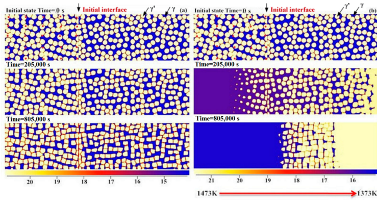
Figure 1.32: Phase-field simulated microstructure evolution of microstructure at the interface between \gamma/\gamma' bond coat and \gamma/\gamma' substrate system (Ni-18.5at.%Al-11.25at.%Cr/Ni-18at.%Al-12at.%Cr) annealed (a) at 1373 K and (b) with an effect of temperature gradient (color bar scale indicates the mole fraction of Al in atom percent, the height of the figure corresponds to 50 \mu\text{m} ; vertical arrow indicates initial BC-substrate interface, BC being on left side and substrate on the right side of the pictures respectively) [175]
