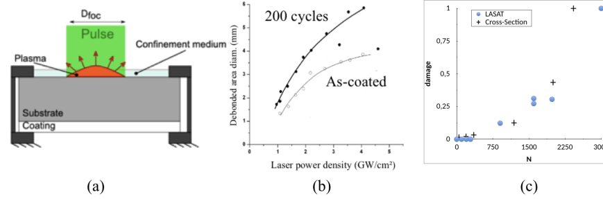
Figure 1.18: Laser Shock Adhesion Testing (LASAT) for the same EB-PVD YSZ, (Ni,Pt)Al coating AM1 single crystal system, (a) set-up and (b) examples of LASAT-2D curves in as-coated condition and after 200 thermal cycles (adapted from [60, 17, 72]), (c) comparison of damage size evolution (normalized) from artificial defects processed by LASAT measured by IR top-surface imaging (non destructive) and on SEM cross-sections (adapted from [186, 110])
