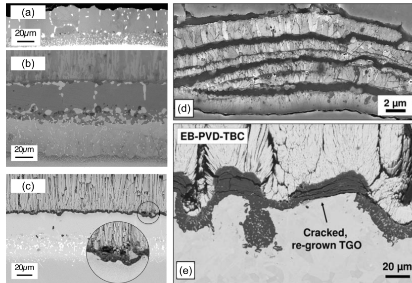
Figure 1.20: Evolution of TGO microstructure for thermal cycling (range 100–1100 °C) for (Ni,Pt)Al BC, (a) after 1000 cycles without TC observed by optical microscope (OM) (adapted from [155]), (b) with EB-PVD TC for N=1200 cycles observed by SEM in BSE mode, (c) SEM image of TBC system from (b) in SE mode (insert corresponds to a zoom of the black circle) (adapted from [113]) and for NiCoCrAlY BC, (d) SEM image in SE mode of oxide fragmentation of a system with APS TC (maximum cycle temperature 1050 °C) and (e) SEM image in SE mode of a system with EB-PVD TC (maximum cycle temperature of 1000 °C) (adapted from [124])
