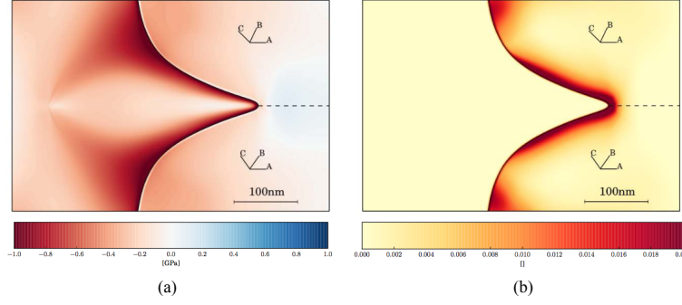
Figure 1.31: Phase field model of 316L oxidation accounting for crystal plasticity and diffusion coupled to stress level, (a) hydrostatic pressure and (b) cumulated plastic strain field [43]
