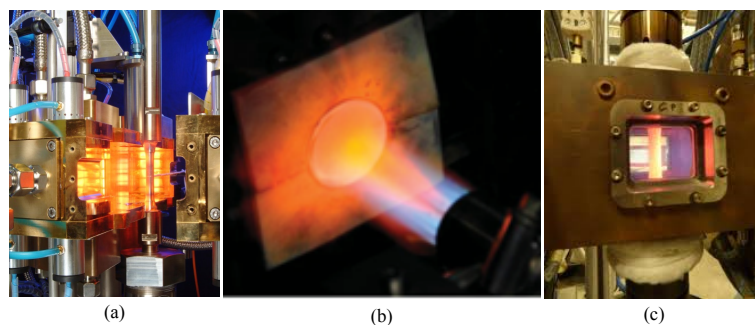
Figure 1.24: TGMF testing of TBC in presence of gradient (a) TGMF [13], (b) Burner rig [103] and (c) Combustion environment in TGMF condition [106]
