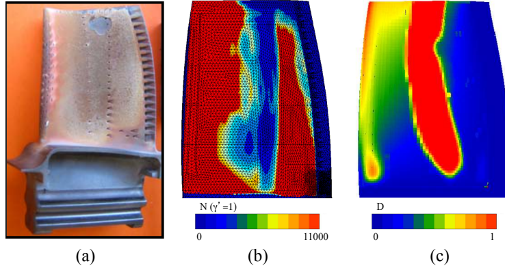
Figure 1.36: High pressure turbine blade, (a) photo of a blade after use in-service [183], (b) phase transformation in bond coat due to thermal exposure, showing the calculated number of cycles to reach a volumic fraction of \gamma'=1 (complete transformation from \beta to \gamma' ) [155], and (c) calculated interfacial damage of the TBC system after thermal exposure [147]
