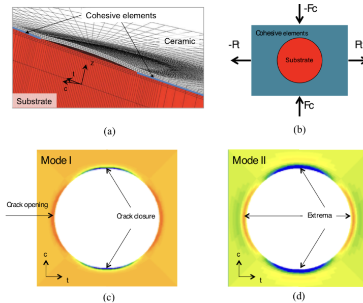
Figure 1.37: Modeling of in-plane biaxial testing (a) perspective view of the half-model highlighting ceramic blister and substrate, (b) schematic top-view without ceramic layer, no cohesive elements are used within the blister making the substrate visible; F_t and F_c indicate in-plane tension and compression, respectively, (c) opening stress component ( \sigma_{zz} ), and (d) shear stress component ( \sigma_{tc} ) highlighting equivalence in shear mode for c and t directions adapted from [159, 158]
