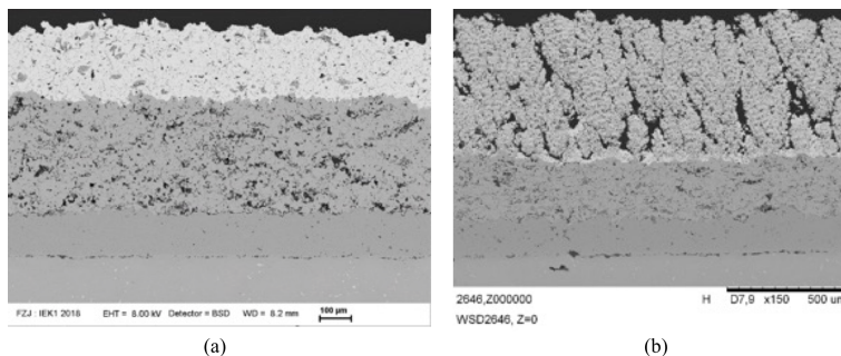
Figure 1.8: SEM micrographs of (a) an APS \text{Gd}_2\text{Zr}_2\text{O}_7/\text{YSZ} and (b) a SPS \text{La}(\text{Al}_{0.25}\text{Mg}_{0.5}\text{Ta}_{0.25})\text{O}_3/\text{YSZ} double layer system.
