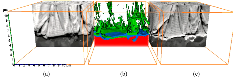
Figure 1.19: Reconstructed volume from FIB-SEM serial sectioning (Box size: 11 \mu\text{m} \times 14.2 \mu\text{m} \times 18.88 \mu\text{m} ). Segmentation of the different phases BC, TGO, TC, and cracks or voids was performed by using images from Backscatter Electron (a) and Secondary Electron (c) detectors. In (b), the BC is displayed in red, the TGO in blue, cracks, respective voids in green, and the TC transparent to allow for viewing the structure of inter-columnar gaps (courtesy of A. Dennstedt).
