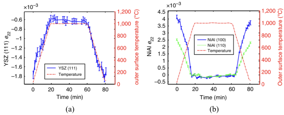
Figure 1.11: In situ measurement of temperature and strain in the loading direction in (a) YSZ layer and (b) in NiAl layer [95]
