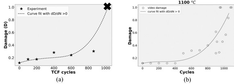
Figure 1.35: Fatigue model based on Paris like crack growth analysis for an APS TBC system under thermal cycling, (a) maximum interfacial crack length, and (b) spalled TC area fraction as a function of cycles number [89]
