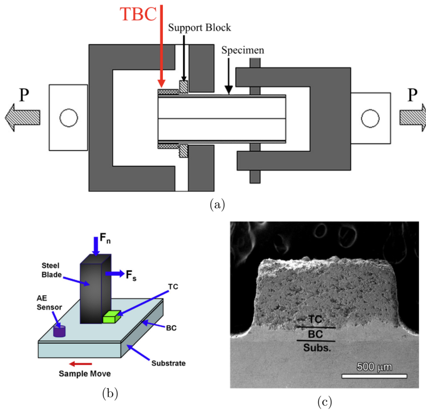
Figure 1.15: (a) Barb test from [74] and (b) shear test from [212], (b) sketch of the set-up and (c) SEM image of the machined specimen, side view
