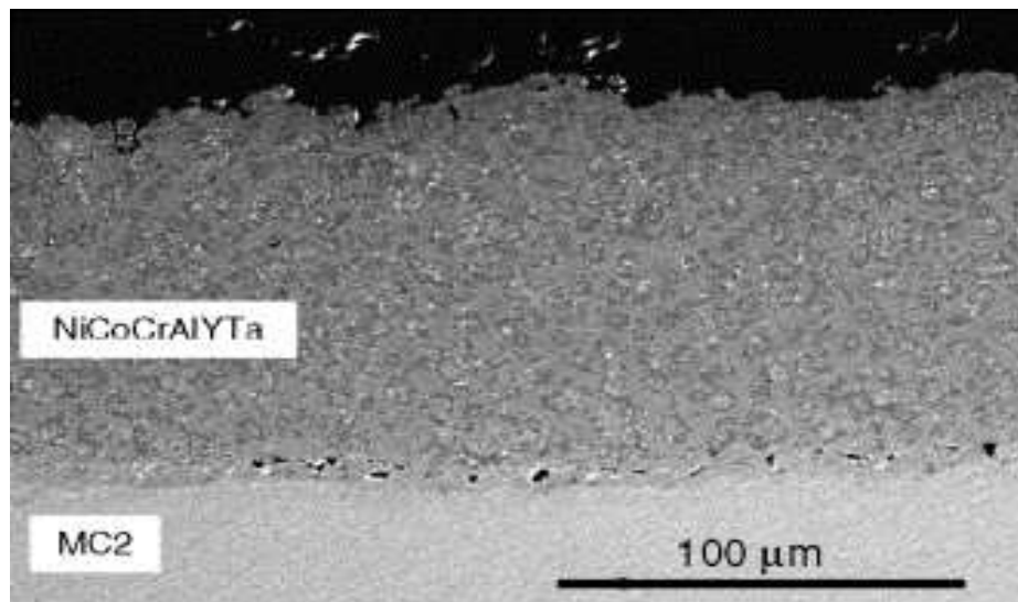
Fig. 1. SEM back scattered electron image of 110- \mu\text{m} thick NiCoCrAlYTaNi coating on MC2 superalloy after vacuum heat treatment.
