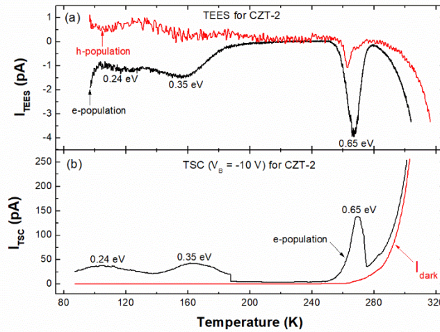
Fig. 6. (a) TEES for CZT-2 sample attained with electron and hole population conditions. (b) TSC spectrum at V_B = -10 V and I_{dark} spectrum for CZT-2.
