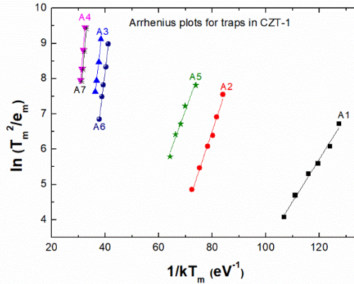
Fig. 2. Arrhenius plots of \ln(T_m^2/e_m) versus 1/kT_m for the peaks A1-A7 observed in the CZT-1 sample.
