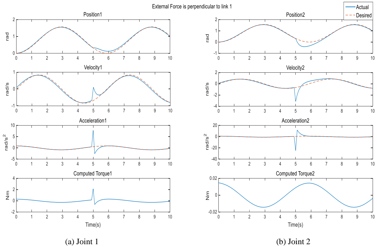
Figure 6. The actual and desired joints' positions, velocities, accelerations and the computed torques when there is external force perpendicular to link 1 and equal to 10 N at time = 5 sec.
