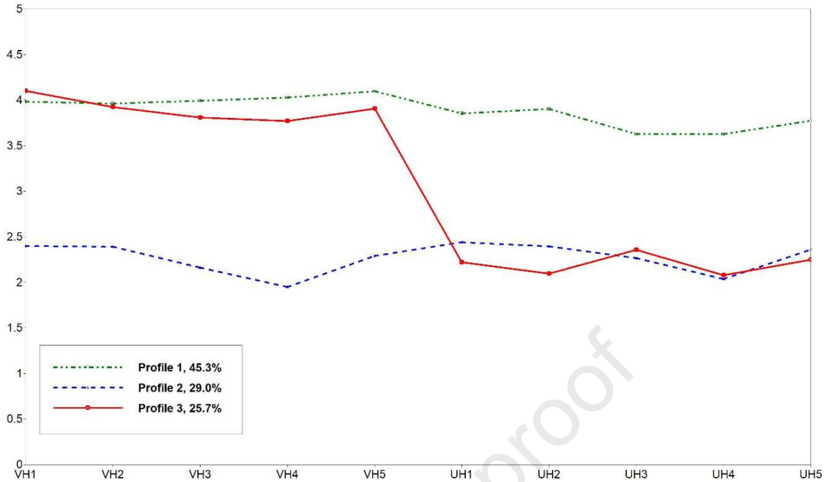
Figure 2. Latent Profiles for Heterogeneous Humanness Perception
