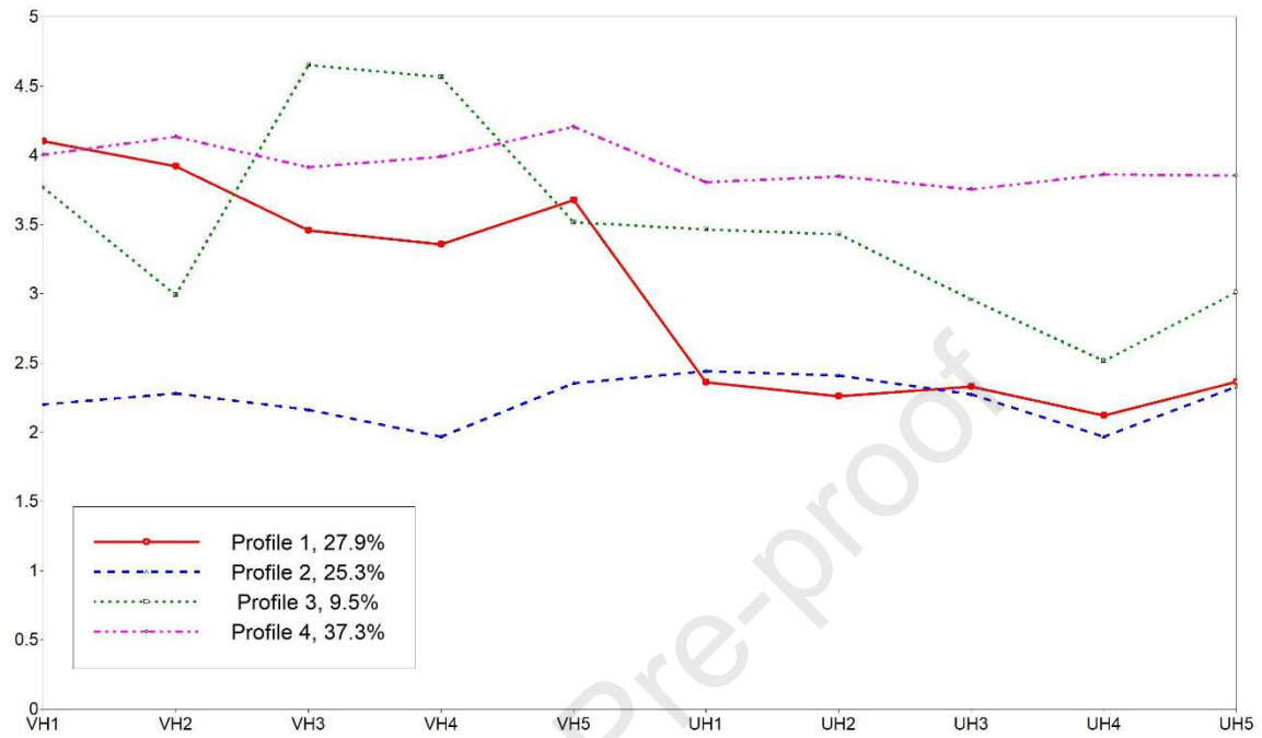
Figure A5. Four-profile Model of LPA with Common Factors
