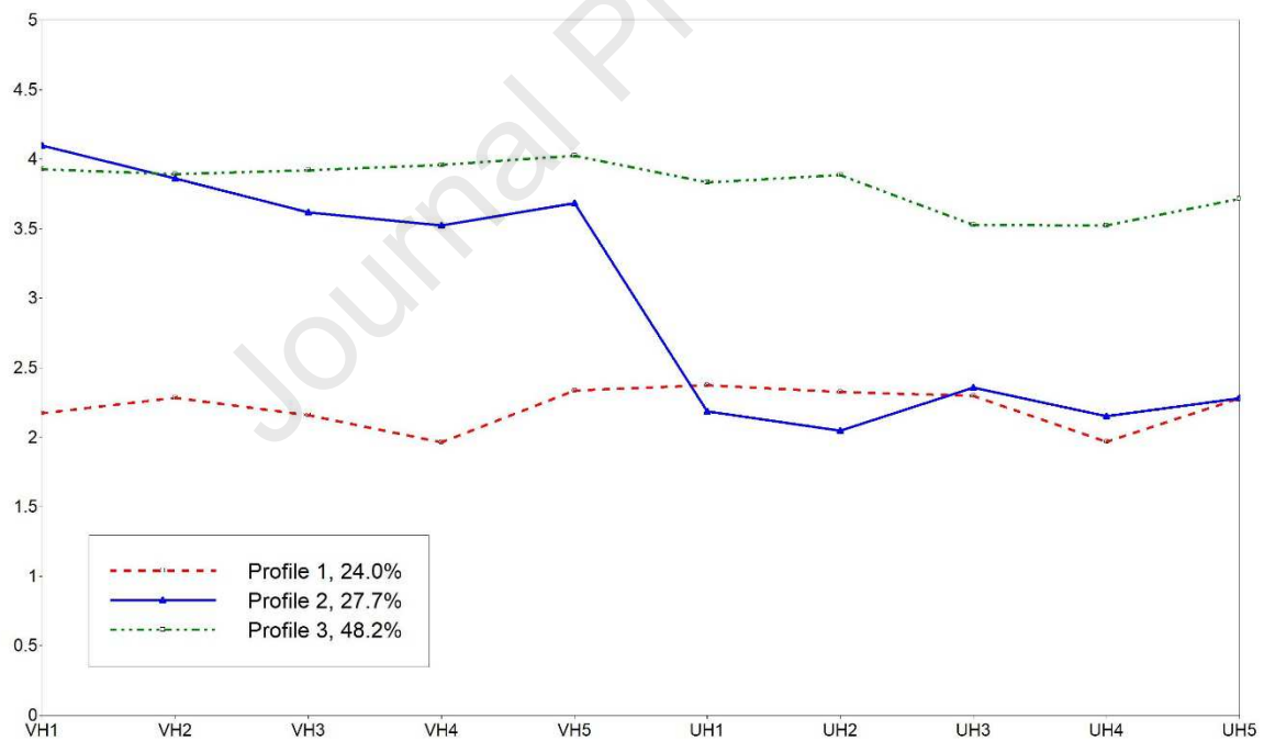
Figure A4. Three-profile Model of LPA with Common Factors
