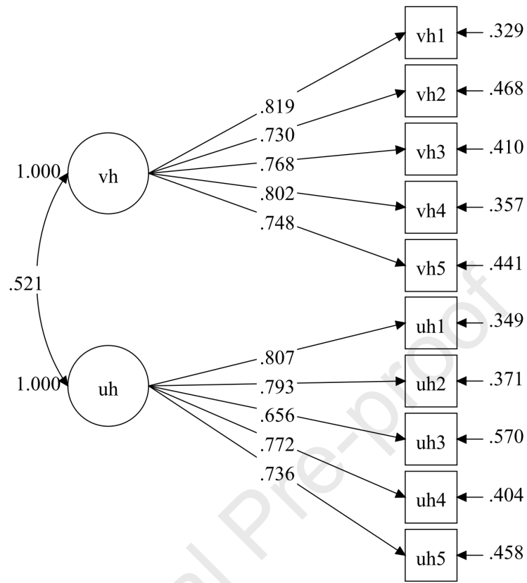
Figure A1. Standardized Solutions of CFA on Humanness Measures (n=625)
