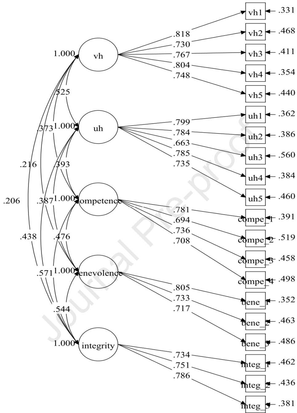
Figure A2. CFA Model with Standardized Estimates
