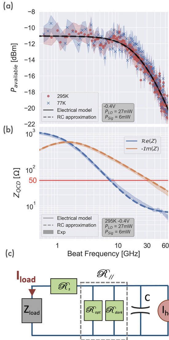
FIG. 4. Available heterodyne power (a) and impedance of the PAR array at 295 K (b) as seen in the Z_{L=0} plane as a function of the frequency. The uncertainty (in shadow) on the power is due to the instability of the QCL sources due to optical feedback. The latter was minimized using an optical isolator. The uncertainty on the impedance comes from the error in determining the distance between the plane L = 0 and the RF probe used during the de-embedding process. (c) RC equivalent model of the PAR array.
