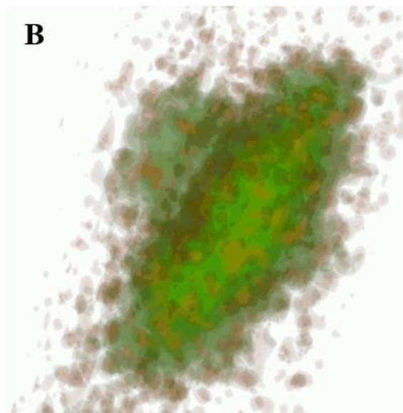
Figure 4: Image of Clostridium perfringens label free cells. Red dots: the endogenous emission of fluorescence from the bacteria. In yellow appears the superimposition of raw and reconstructed signals. Green: reconstructed signal of
