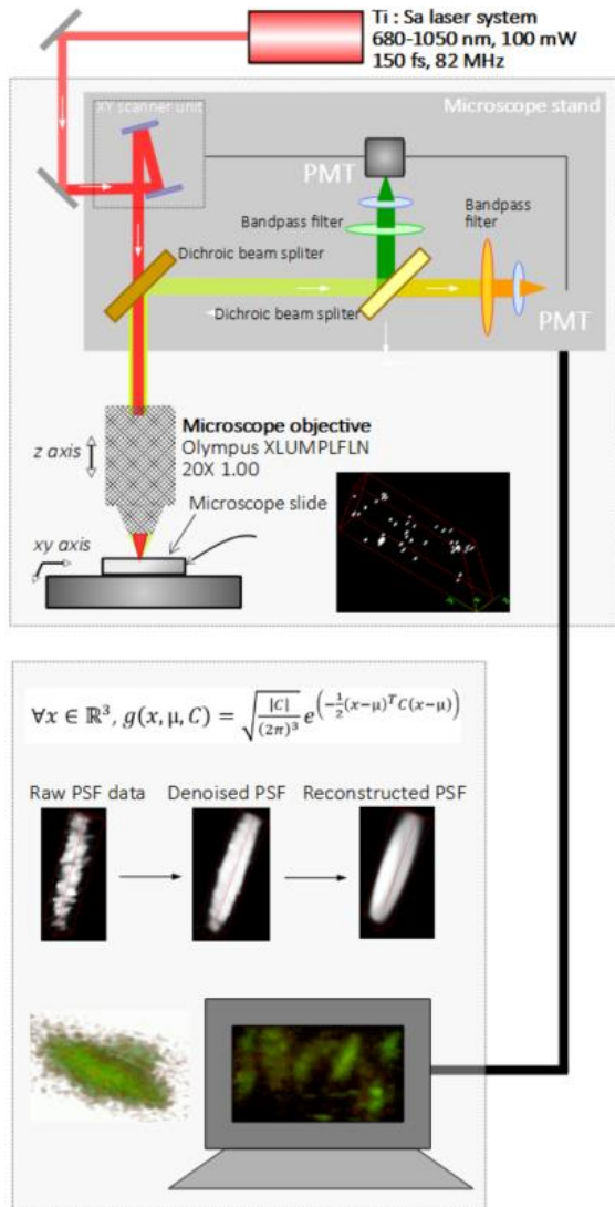
Figure 1: Experimental setup for recording the multiphoton images of bacteria, associated with a computational strategy for 3D image recovery.
