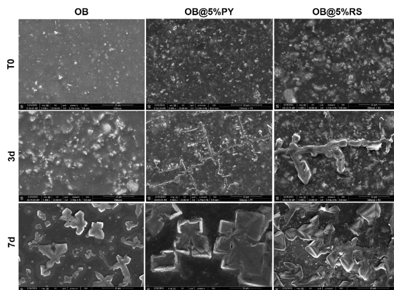
Figure 6. Representative scanning electron microscopy images at 5000 \times magnification. The morphologies of OB, OB@5%RS and OB@5%PY surfaces were analyzed in dry condition (T0); and after 3 and 7 days in PBS at 37 °C.
