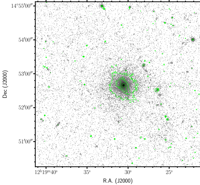
Fig. 2. H\alpha + [NII] contours (at a surface brightness level of \Sigma(H\alpha + [NII]) = 3 \times 10^{-17}, 1 \times 10^{-16}, 2 \times 10^{-16}, 1 \times 10^{-15} \text{ erg s}^{-1} \text{ cm}^{-2} \text{ arcsec}^{-2} ) plotted over the UVIT NUV image in the Silica15 band of the galaxy NGC 4262 (grey).
