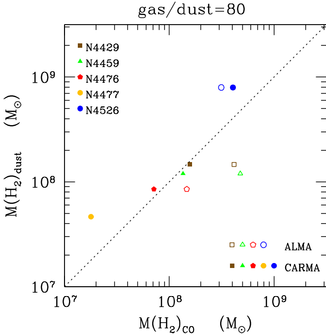
Fig. 20. Relation between the molecular gas mass derived using the total dust mass and assuming a gas-to-dust ratio of G/D = 80 and the molecular gas mass derived using CO observations for galaxies with ALMA (empty symbols) and CARMA (filled symbols) data. The different galaxies are indicated by different symbols. The dotted line shows the expected relation for a gas-to-dust ratio G/D = 80 .
