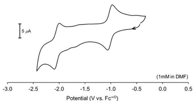
Figure 2. Cyclic voltammogram of a DMF solution of Co II Fe II (1 mM); electrolyte: 0.1 M (\text{Bu})_4\text{NClO}_4 ; reference: \text{Ag}/\text{AgNO}_3 ; counter: Pt wire; scan rate: 100\text{ mV s}^{-1} .
