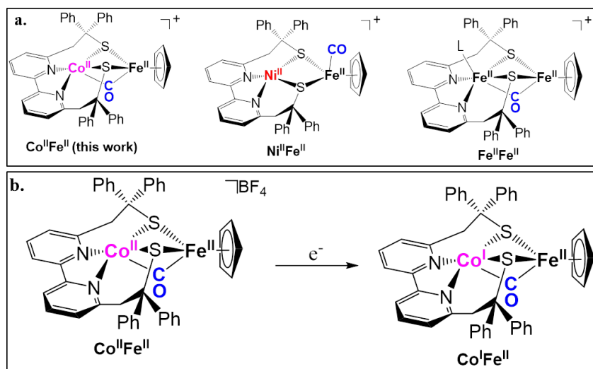
Scheme 1. (a) Family of dinuclear model complexes ( CoFe (this work), NiFe , 11 and FeFe 10 with L = CO or solvent). (b) Reduction reactivity of the Co^II Fe^II complex described in this work.
