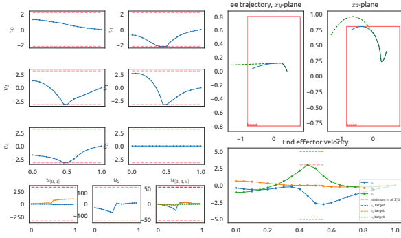
Fig. 5. Joint angles (upper left), joint velocities (middle left), controls (lower left), end-effector trajectory (upper right) and velocity (lower right) for the throwing motion on UR10. The ball trajectory is displayed with dashed green lines on the upper-right plots. Both the velocities, controls and end-effector position satisfy their respective bounds, displayed in red. The minimum target end-effector velocity is also satisfied.
