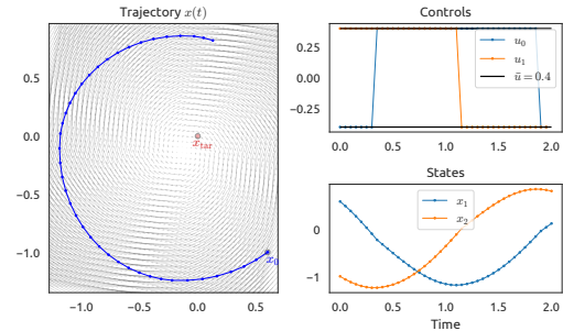
Fig. 3. A approximates the continuous-time matrix A_c = \begin{bmatrix} 0.4 & 2 \\ -2 & 0.4 \end{bmatrix} and same c , the target is located near a repulsive equilibrium. Then, even with the same bound \bar{u} = 0.4 , the target is not reached. The obtained control is a bang-bang or on/off control.
