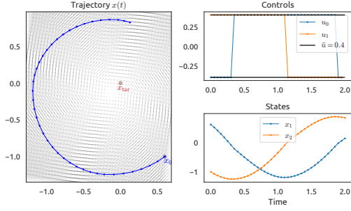
Fig. 3. A approximates the continuous-time matrix A_c = \begin{bmatrix} 0.4 & 2 \\ -2 & 0.4 \end{bmatrix} and same c , the target is located near a repulsive equilibrium. Then, even with the same bound \bar{u} = 0.4 , the target is not reached. The obtained control is a bang-bang or on/off control.
