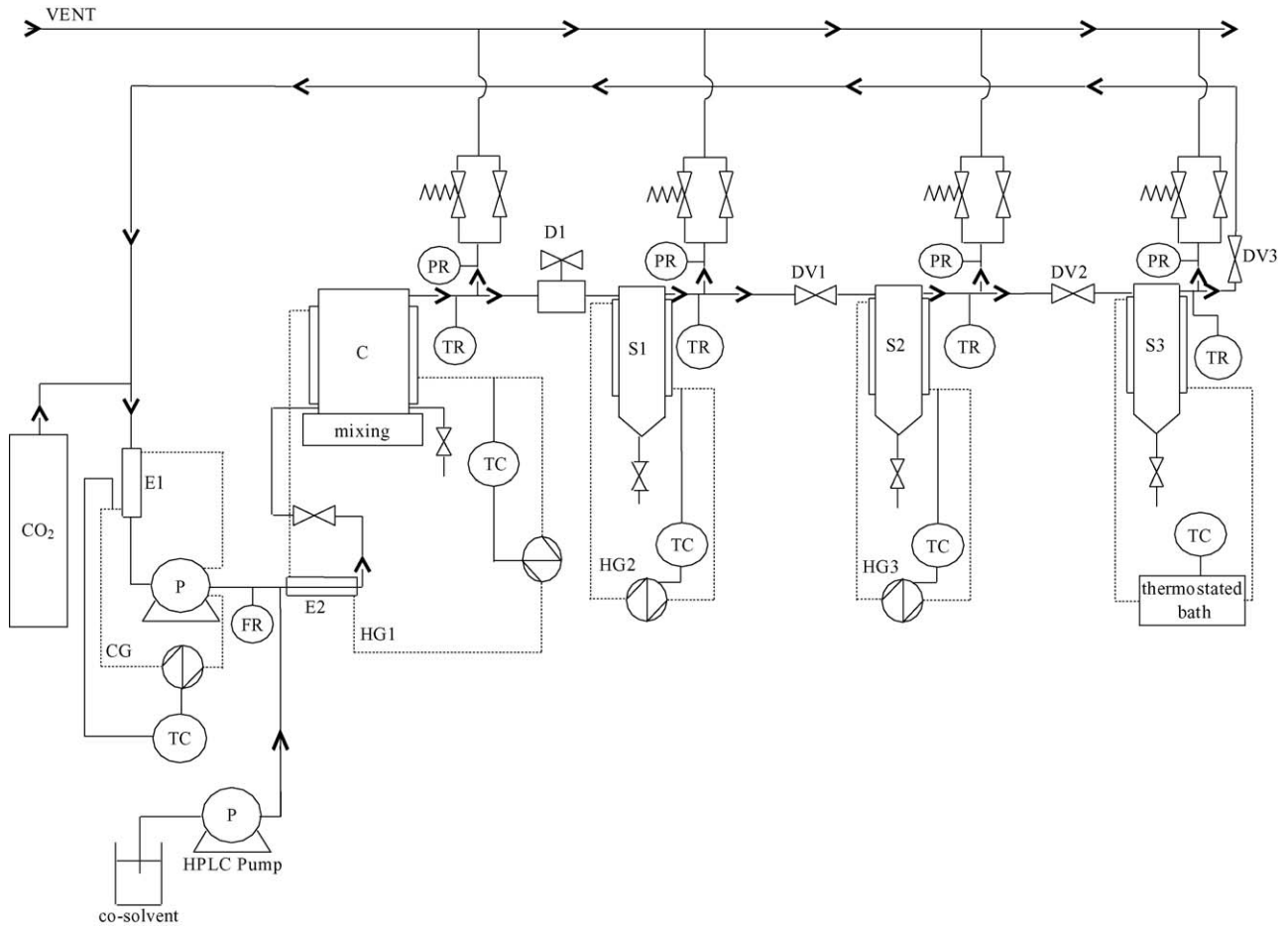
Fig. 1. Pilot SF200. C: mixing chamber; S1, S2, S3: separators; CG: cooling group; HG: heating group; PR: pressure recording; TC: temperature control; TR: temperature recording; D1: back-pressure regulator; DV1, DV2, DV3: depressurisation valves; E1: condenser; E2: evaporator.
