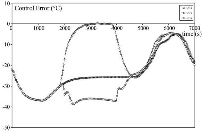
Fig. 13. Relatives control errors evolution: PFCs controller.
