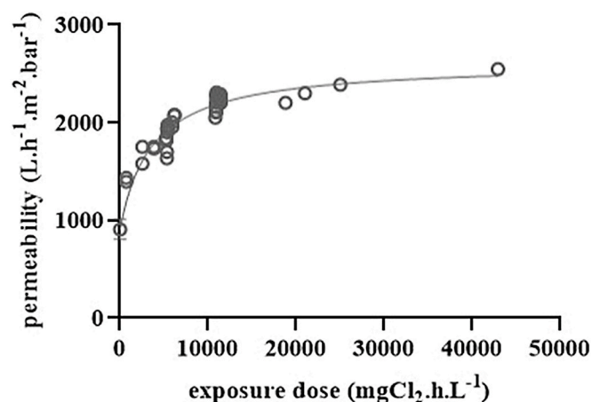
Fig. 3. Variation of permeability as the function of the chlorine exposure dose ( \text{mgCl}_2\cdot\text{h}\cdot\text{L}^{-1} ) after static immersion [ 30\,\text{mgCl}_2\cdot\text{L}^{-1} ; pH 7.5].
