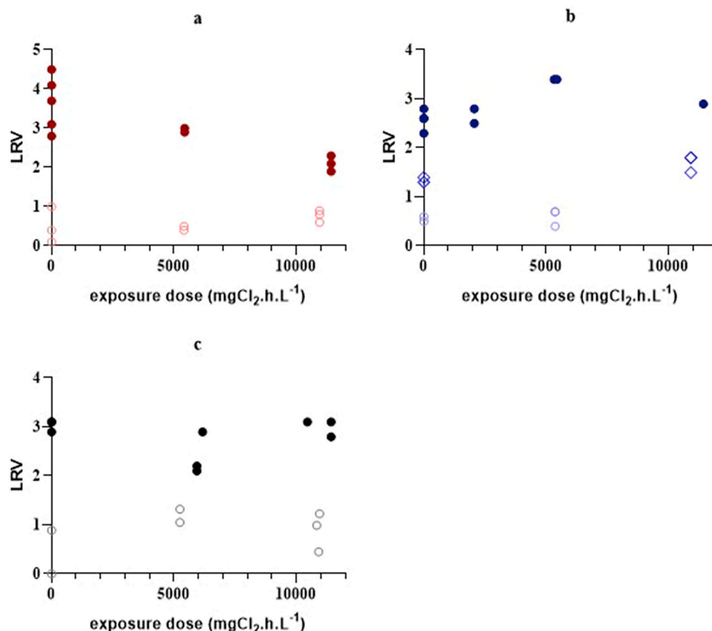
Fig. 4. Variation of LRV as the function of the chlorine exposure dose (mgCl 2 .h.L -1 ) after static immersion [30 mgCl 2 .L -1 ; pH 7.5] regarding retention of a) ADV 41 b) CV-B5 c) MS2 phages, at various feed concentrations ((●) for high feed concentrations, (◇) for intermediate feed concentrations, (○) for low feed concentrations). Each point represents a single experiment.
