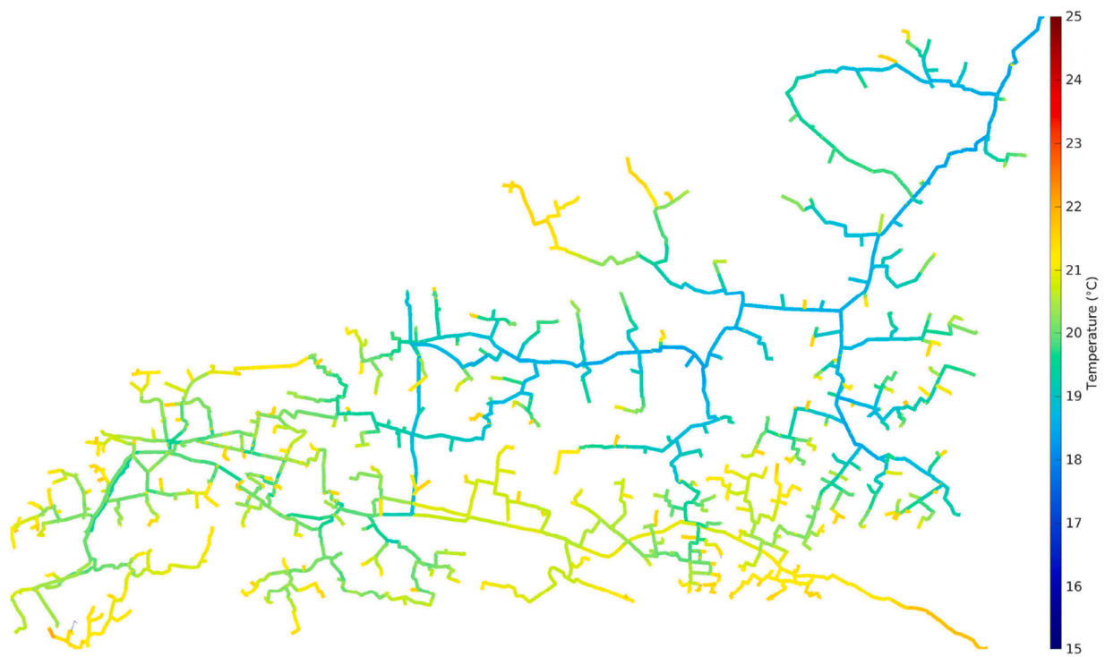
Fig. 12. Modeled water temperature in the raw water network (presented in 2) on the 30th of June 2018 at midday (soil temperature is .21.6°C).
