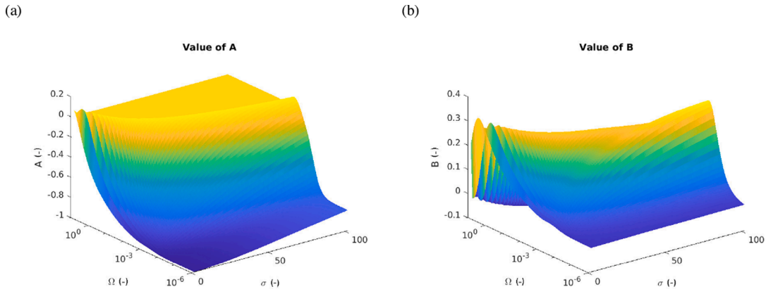
Fig. 16. Value of parameter A and B of Barletta's method [14] according to \Omega . and \sigma .
