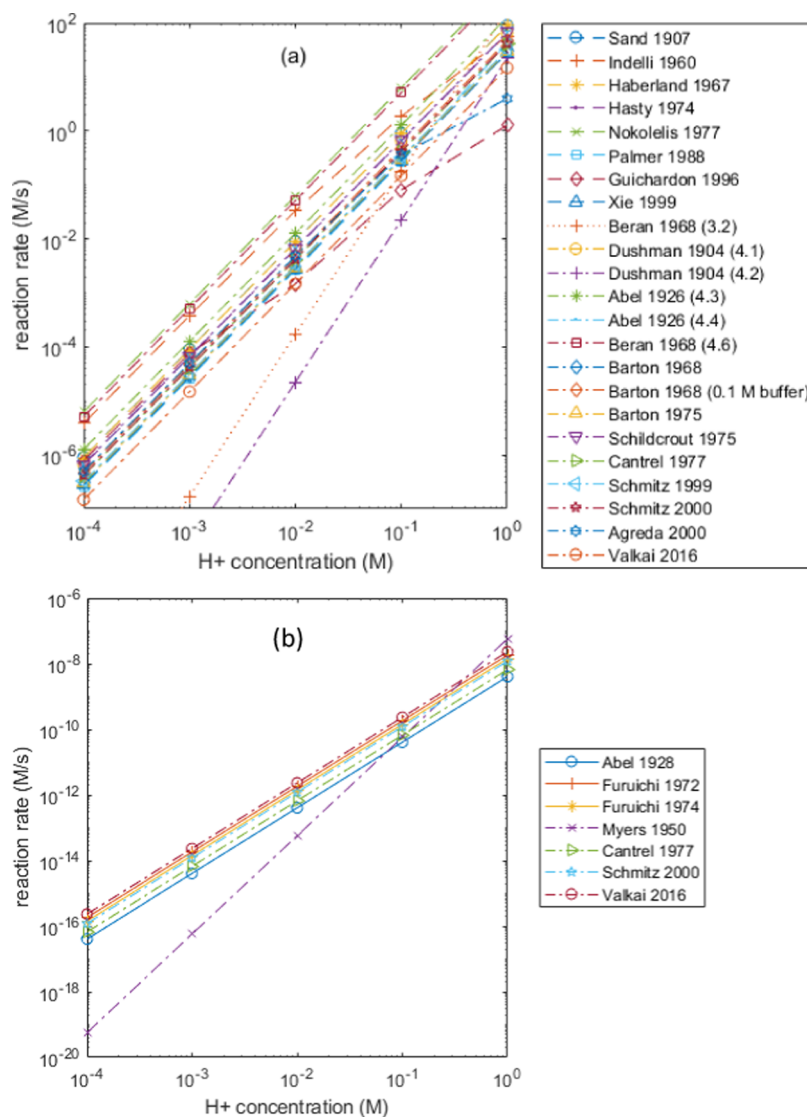
Figure 2. Influence of H^+ concentration on rate laws: (a) [IO_3^-] = 10^{-5} \text{ M} ; [I^-] = 0.01 \text{ M} ; (b) [IO_3^-] = 10^{-5} \text{ M} ; [I^-] = 10^{-8} \text{ M} .
