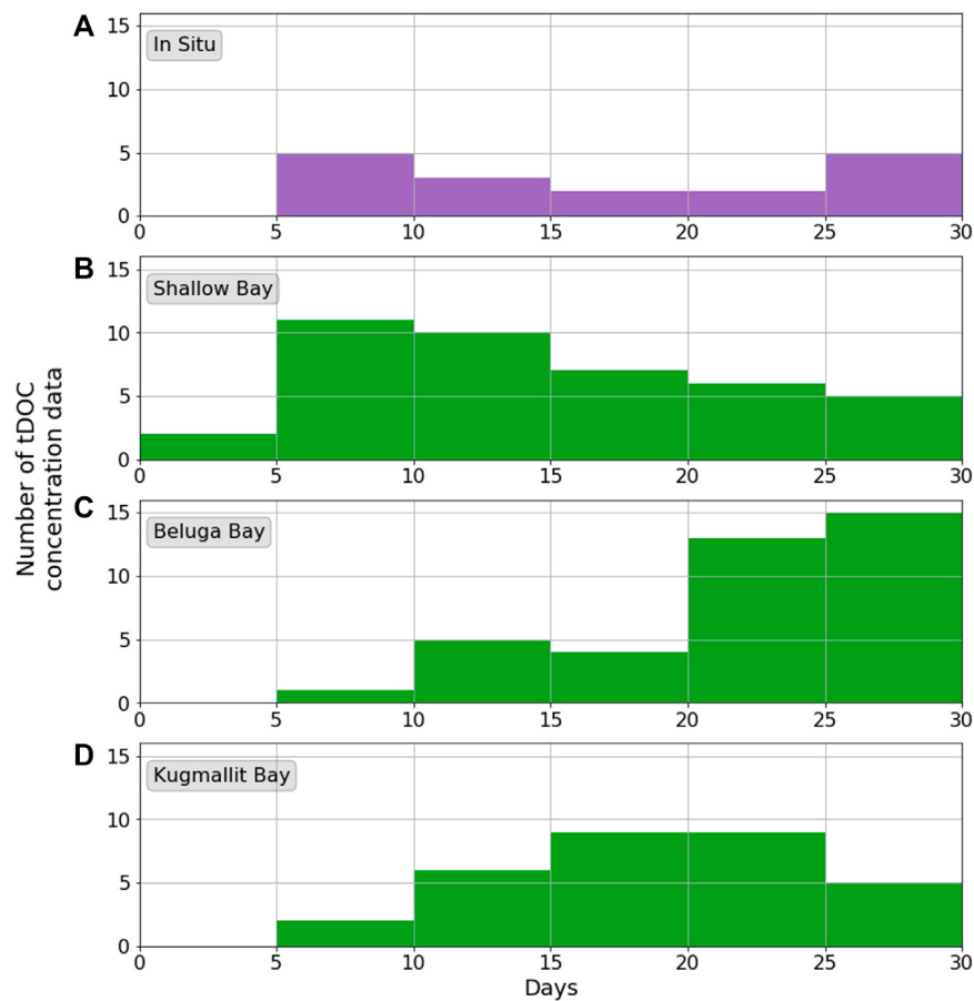
FIGURE 7 | Temporal distribution in June (2003–2017) of the (A) \text{tDOC}_{\text{in situ}} concentrations, and (B) \text{tDOC}_{\text{sat}} concentrations for Shallow Bay, (C) Beluga Bay and (D) Kugmallit Bay.
