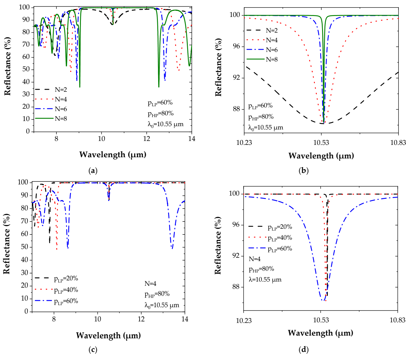
Figure 5. Reflectance spectrum of microcavities based on symmetric PGe Bragg mirrors with: (a,b) porosities p_{LP} = 60\% and p_{HP} = 80\% while varying N ; (c,d) N fixed to 4, porosities p_{HP} = 80\% and varying p_{LP} ; (d) the magnification of the spectra around the resonance wavelength.
