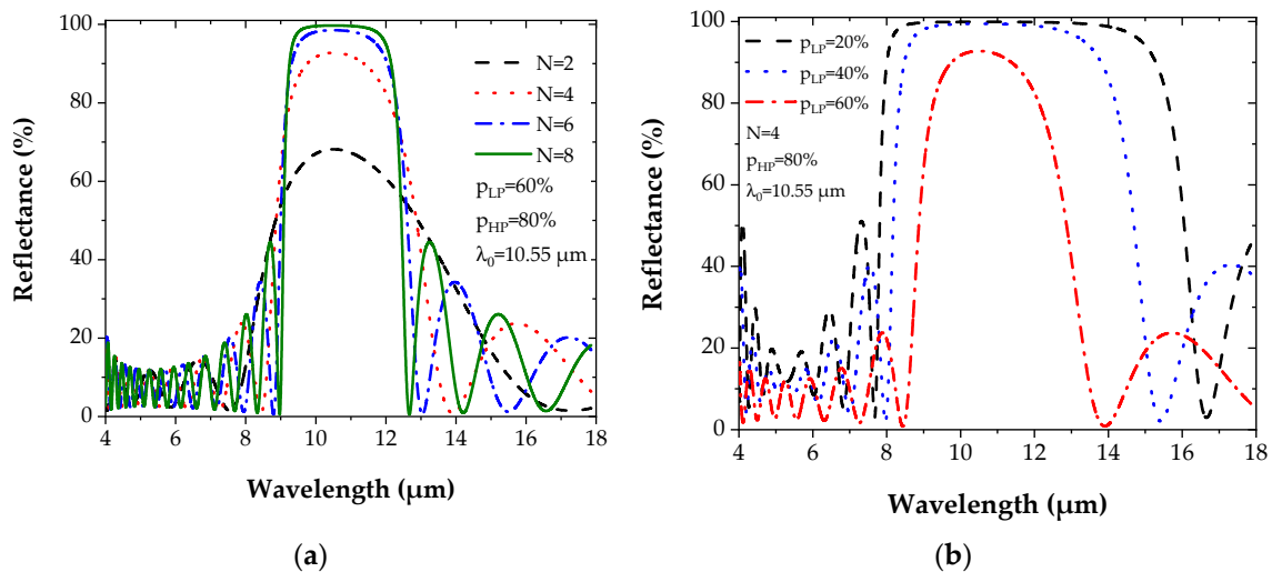
Figure 4. (a) The Bragg reflector for PGe materials with (a) porosities p_{LP} = 60\% and p_{HP} = 80\% while varying N . (b) Reflectance spectrum when N is fixed to 4, porosities p_{HP} = 80\% , and varying p_{LP} .
