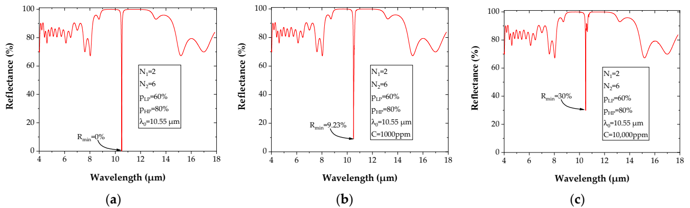
Figure 8. Reflectance spectrum of asymmetric microcavity, for PGe materials: without gas (a) and with SF 6 concentrations in air of (b) 1000 ppm, and (c) 10,000 ppm.
