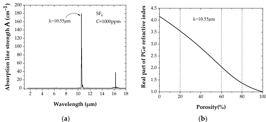
Figure 1. (a) Mid-IR absorbance spectrum of SF 6 (for a SF 6 concentration of 1000 ppm in air). (b) Dependence of the real part of the PGe refractive index on porosity.
