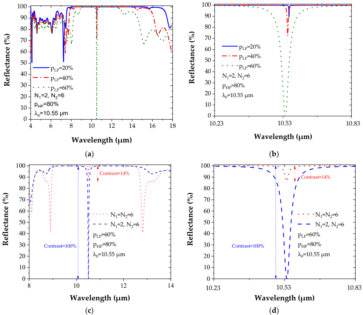
Figure 7. (a,b) Reflectance spectrum of asymmetric microcavities: N_1 = 2 and N_2 = 6 , porosities p_{HP} = 80\% and varying p_{LP} . (c,d) Comparison between the reflectance spectrum of the symmetric ( N_1 = N_2 = 6 ) and asymmetric microcavities ( N_1 = 2 and N_2 = 6 ) for p_{HP} = 80\% and p_{LP} = 60\% .
