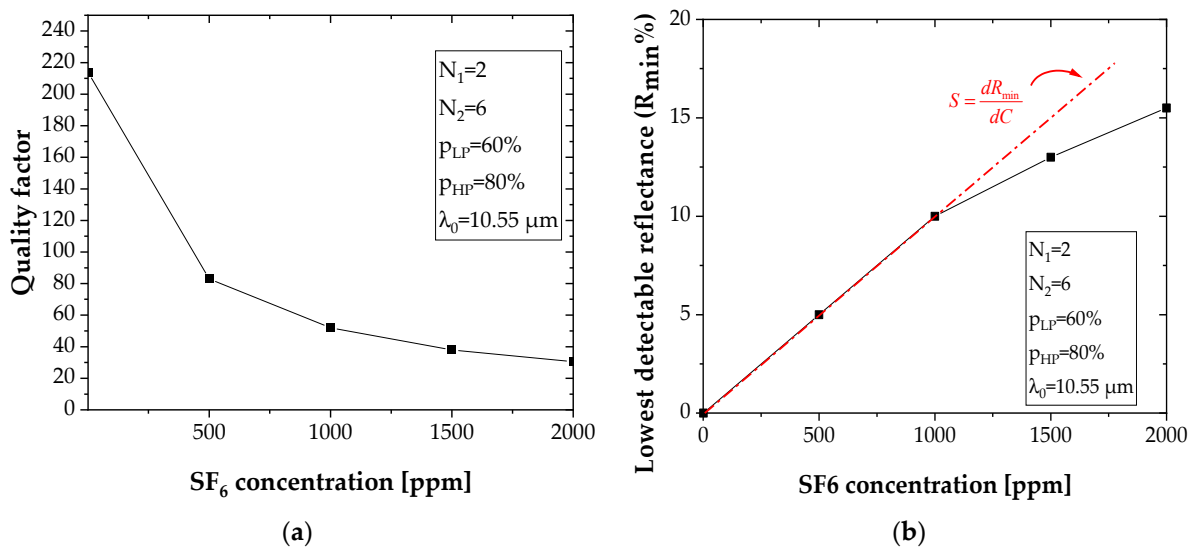
Figure 9. (a) Quality factor Q as a function of SF 6 concentration. (b) The lowest detectable reflectance as a function of concentration of target molecules.
