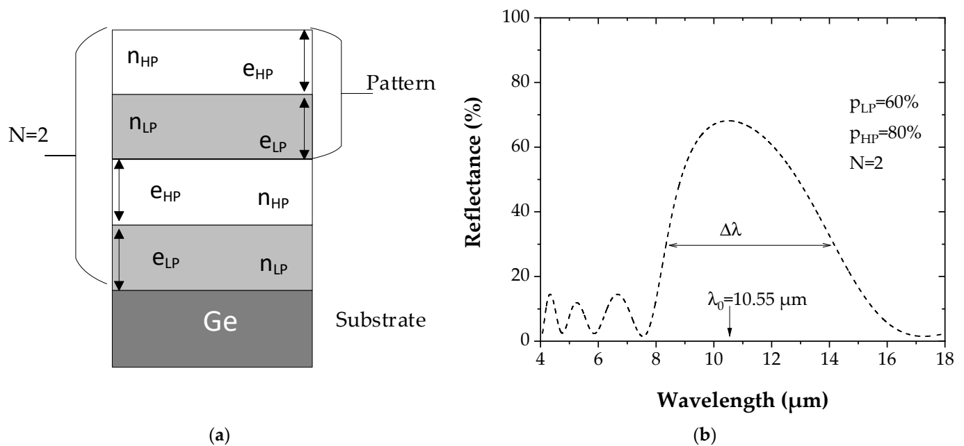
Figure 2. (a) Schematic of a PGe Bragg reflector made of a repeated pattern constituted by alternating a layer of low porosity (refractive index n_{LP} and thickness e_{LP} ) and a layer of high porosity (refractive index n_{HP} and thickness e_{HP} ). In this case, the pattern is repeated twice ( N = 2 ). (b) Calculated reflectance spectrum of the corresponding PGe Bragg reflector, with values of 60% and 80% for the low and the high porosities, respectively.
