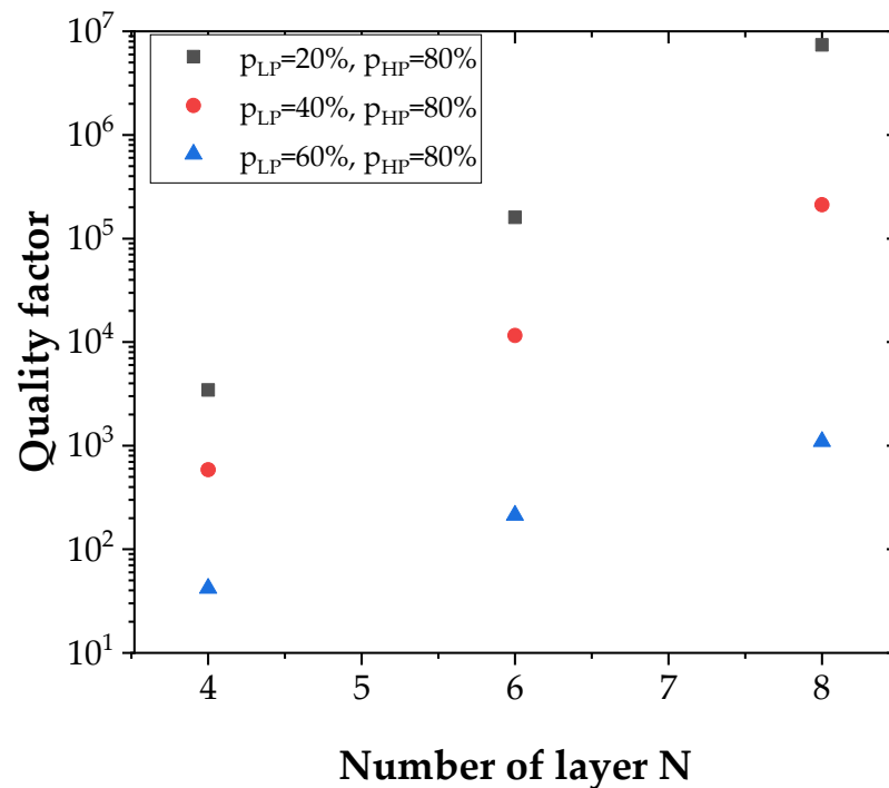
Figure 6. Quality factor Q as a function of layer number N for the microcavities studied.
