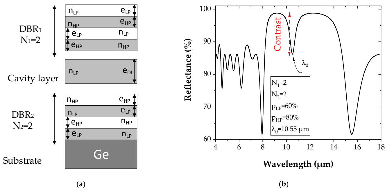
Figure 3. (a) Schematic of a PGe microcavity reflector constituted of a Fabry–Perot layer cavity of low porosity (refractive index n_{LP} and thickness e_{DL} ) sandwiched by two DBRs. The two DBRs are made of a pattern of low (60%) and high porosity (80%) layers with a refractive index n_{LP} and n_{HP} and a thickness e_{LP} and e_{HP} , respectively, and repeated in this case two times. (b) Calculated reflectance spectrum of the PGe microcavity reflector with values of 60% and 80% for the low and the high porosities, respectively.
