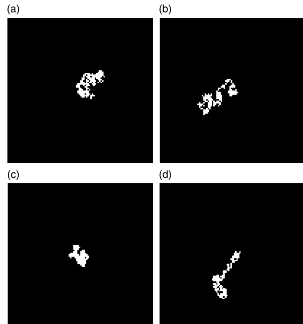
Fig. 7. Examples of spalls simulated with N_G = 250 growth steps shown here on a 100×100 pixel grid.
