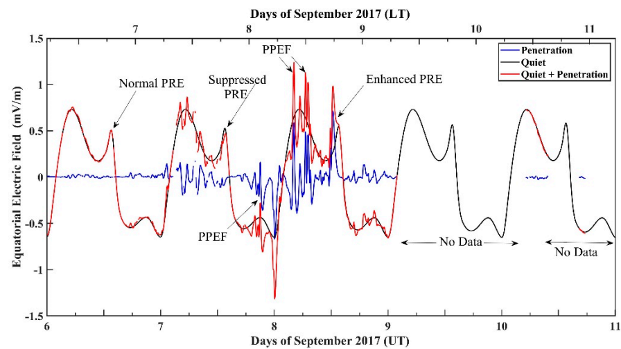
Figure 4. Effects of the prompt penetration electric fields (PPEFs) towards the enhanced duskside PRF calculated from the real-time prompt penetration electric field model (PPEFM; https://geomag.colorado.edu/real-time-model-of-the-ionospheric-electric-fields , accessed on 18 January 2022) [78] over the Indian longitude ( 78^\circ E) in the main phase of the storm during 6–10 September 2017. The black line shows the background quiet-time electric field, whereas the blue and red lines indicate the prompt penetration electric field and the total electric field (the sum of quiet-time and prompt penetration electric fields), respectively.
