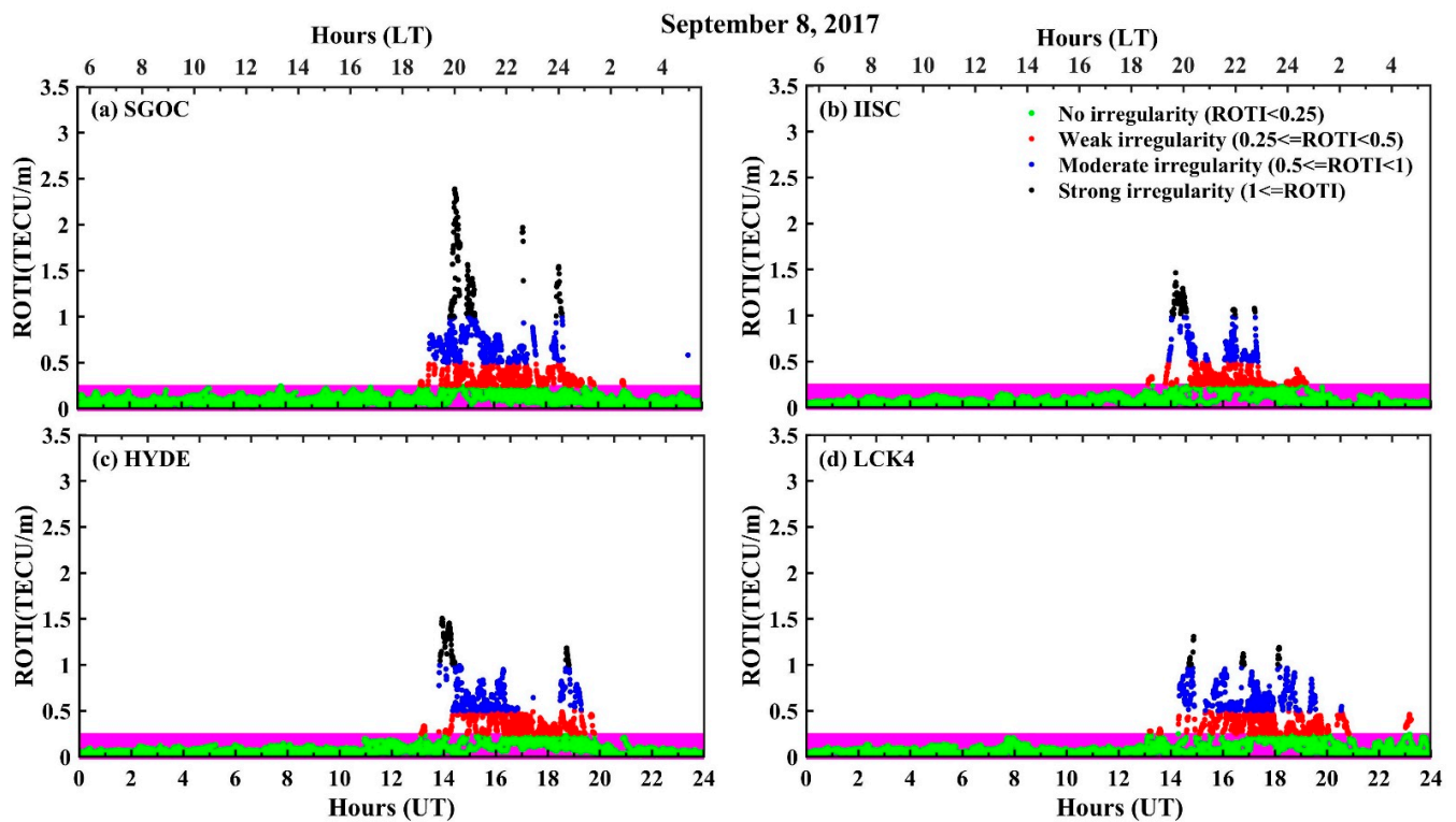
Figure 6. Classification of the ionospheric irregularities based on the ROTI values at (a) SGOC, Colombo, (b) IISC, Bangalore, (c) HYDE, Hyderabad, and (d) LCK4, Lucknow on the geomagnetic storm day (8 September 2017). The criteria for the classification of the irregularities is chosen as (i) no irregularity ( \text{ROTI} < 0.25 ; in green); (ii) weak irregularity ( 0.25 \leq \text{ROTI} < 0.5 ; in red); (iii) moderate irregularity ( 0.5 \leq \text{ROTI} < 1 ; in blue); and (iv) strong irregularity ( \text{ROTI} \geq 1 ; black). The shaded portion with \text{ROTI} < 0.25 is masked out in this study.
