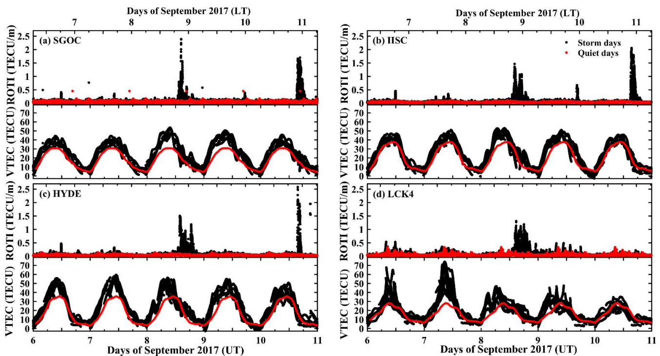
Figure 5. Variation of the VTEC and ROTI parameters at (a) SGOC, Colombo; (b) IISC, Bangalore; (c) HYDE, Hyderabad; and (d) LCK4, Lucknow, during the storm period from 6–10 September 2017 (in black), superimposed with the corresponding quiet-time reference values (in red).
