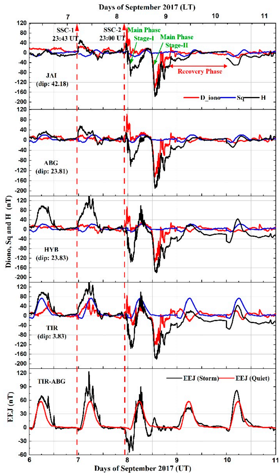
Figure 3. Variation of the horizontal magnetic field component H (in black), superimposed with the regular Sq variation (in blue) and D_{iono} component (in red) that corresponds to the disturbances due to ionospheric currents registered at all four magnetometer observatories (top 4-panels) during the storm period from 6–10 September 2017. The bottom panel shows the variation of the EEJ proxy index during the storm period (in black) superimposed with the averaged quiet-time reference level (in red).
