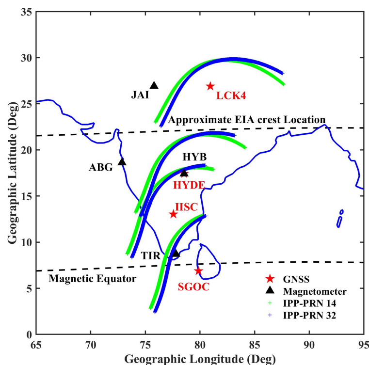
Figure 1. Geographic locations of the magnetometer observatories (black triangle) and the IGS GNSS stations (red star) in the Indian longitude sector considered in the study. The dashed horizontal contour lines represent the approximate positions of the magnetic equator and northern EIA crest. The ionospheric piercing point (IPP) locations for the GPS PRNs, 14 and 32, during the storm on 8 September 2017 are indicated by the green (+) and blue (+) curves, respectively.
