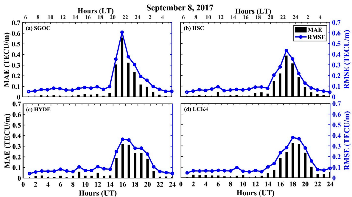
Figure 7. Diurnal maximum absolute error (MAE) and root mean square error (RMSE) of ROTI at (a) SGOC, Colombo, (b) IISC, Bangalore, (c) HYDE, Hyderabad, and (d) LCK4, Lucknow on the geomagnetic storm day (8 September 2017), with respect to the averaged quiet-time reference level.
