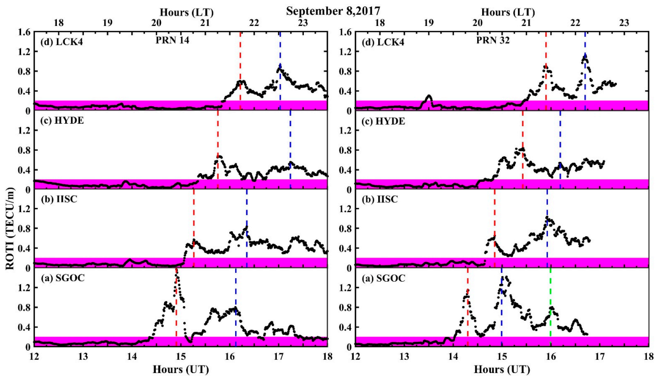
Figure 8. Spatiotemporal variation of the plasma irregularities marked from the simultaneous ROTI observations from PRN-14 and PRN-32 GPS satellite signals at (a) SGOC, Colombo, (b) IISC, Bangalore, (c) HYDE, Hyderabad, and (d) LCK4, Lucknow on the geomagnetic storm day (8 September 2017), respectively arranged from bottom to top. The vertical dotted lines indicate the timestamps of corresponding ROTI peaks at all stations. The pink-colored shaded portion at the bottom indicates the masked-out ROTI values ( \text{ROTI} < 0.25 ), wherein the TEC fluctuation is assumed to be absent.
