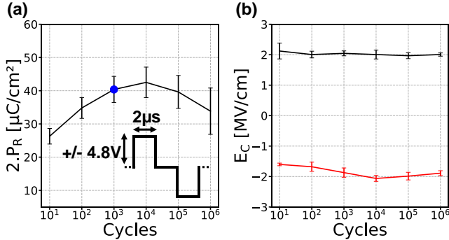
Figure 2: (a) Remanent polarization 2.P R and (b) coercive field E C along cycling measured on 1T-1C structures cycled with square electrical pulses (4.8V 2µs). The mean value on 5 dies tested in this paper is extracted. The blue dot represents the median 2.P R considered in the 16kbit arrays on the same wafer, i.e. after 1000 cycles 4.8V 2µs.
