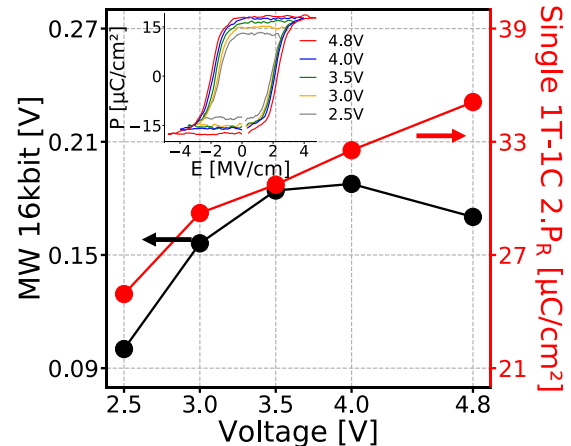
Figure 11: Memory Window at 16kbit scale as a function of programming/reading voltage from 4.8V down to 2.5V at constant 2 \mu s pulse width ( 0.36\mu\text{m}^2 TiN/HfO 2 :Si/TiN capacitors) compared with 2.P_R after wake-up measured on a stand-alone 1T-1C capacitor.
