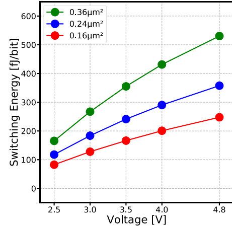
Figure 16: Median ferroelectric switching energy per bit calculated with equation (2), using \epsilon_{\text{HfO}_2:\text{Si}}=30 and C_{\text{BL}}=280\text{fF} .
