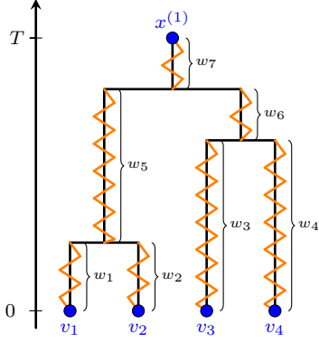
Figure 4.3: Illustration of the centered MORAN process where |k_{4,T}| = 1 .
