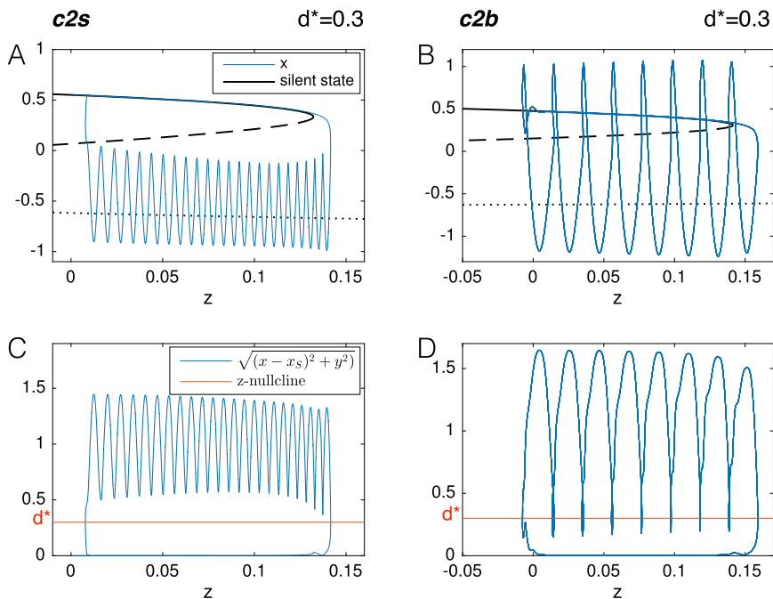
Fig. 7 Slow dynamics. We choose class SN/SH c2s ( left panel ) as an example for classes in which the silent state is outside the limit cycle. In A it can be observed that the projections of the oscillations on the x-axis can be separated from that of the silent state. This is not true for classes in which the silent state is encircled by the limit cycle, as in class SN/SH c2b ( right panel ). For this class the projection of the oscillations on the x-axis cannot be separated by that of the silent state ( B ). This separation becomes possible if we use, instead of the x -variable of the bursting trajectory, the distance of the latter from the silent state ( \sqrt{(x - x_s)^2 + y^2} ) ( C–D ). In C and D we added in red the z -nullcline
