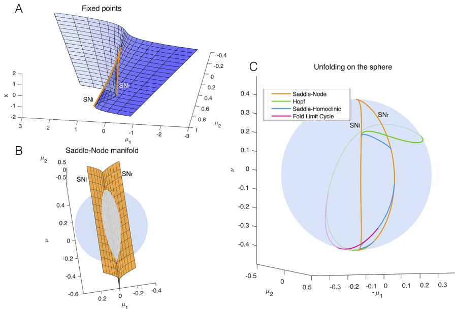
Fig. 3 Unfolding of the deg. TB singularity, focus case. A The fixed points of the system are found for y_0 = 0 , x_0^3 + \mu_2 x_0 - \mu_1 = 0 . The blue surface represents x_0 plotted against the two parameters \mu_1 , \mu_2 . In orange are marked the curves of saddle-node bifurcations at which the saddle solution (i.e. the middle branch) collides with the focus in the upper or lower branch and annihilates. B The manifold of the saddle-node bifurcation (in orange) is plotted in the three dimensional unfolding parameters space together with a sphere of radius R = 0.4 centered at the origin of the parameter space (\mu_1, \mu_2, v) = (0, 0, 0) . The intersection between the surface of saddle-node bifurcations and the spherical surface gives a curve of saddle-node bifurcation. C The bifurcation curves obtained at the intersection between the sphere and all the bifurcation surfaces of the unfolding. In this figure we do not separate between supercritical and subcritical Hopf (both in green) and between saddle node and SNIC (both in orange)
