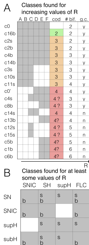
Fig. 19 Existence and complexity of classes. A The letters from A to F refer to the stages of topological equivalence identified in Fig. 15 for increasing R . Some of the classes that were found for small R disappeared far from the codim-3 singularity, while new classes appeared when exploring the codim-4 unfolding. The figure shows the lifespan of each class as a function of R (gray indicates the existence of a class). For each class we report the smallest codimension of the local singularity in which unfolding the class first appears. This can be used as a measure of complexity. We identified hysteresis-loop bursters of complexity 2, 3 and 4 (green, orange and red). For the classes with a question mark, further investigation is needed to establish their complexity in terms of codimension. As an additional element to understand the complexity of a class, we report the minimum number of bifurcation curves that the path for that class here identified has to cross, which may also affect whether an arc of great circle can be used as a path (last column, 'y' (yes) if the great circle 'g.c.' can be used, 'n' (no) otherwise). B The table summarizes the hysteresis-loop bursting classes present in our model, considering also changes in R . The letters 's' and 'b' indicate whether the silent state is, respectively, outside or inside the limit cycle of the active phase
