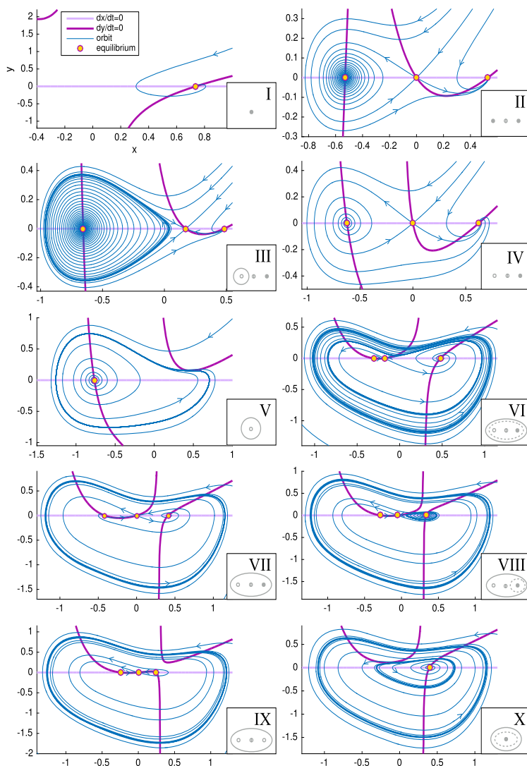
Fig. 5 Phase flows. For each region of the unfolding, labeled with a Roman numeral in Fig. 4, we show the nullclines of Eq. (2) in light and dark purple. Fixed points at the intersection of the nullclines are marked with yellow dots. Flows are shown in blue. Nullclines and fixed points are computed analytically, flows are obtained through numerical simulations in Matcont
