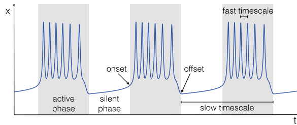
Fig. 1 Bursting activity. Bursters are characterized by the alternation between active (gray boxes) and silent (white) phases. In fast–slow bursters we can distinguish two rhythms: one within the active phase, the fast time scale, and the other between active and silent phases, the slow time scale. Oscillations start at the onset of the active phase and terminate at its offset
