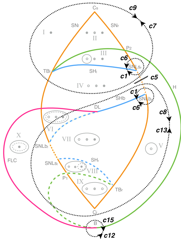
Fig. 12 Paths for slow-wave bursters. We show examples of closed paths for the slow-wave bursting classes ( dotted black curves ). Paths for classes for which an hysteresis-loop counterpart exists are not shown, the hysteresis-loop path can, in fact, be used also for slow-wave bursting
