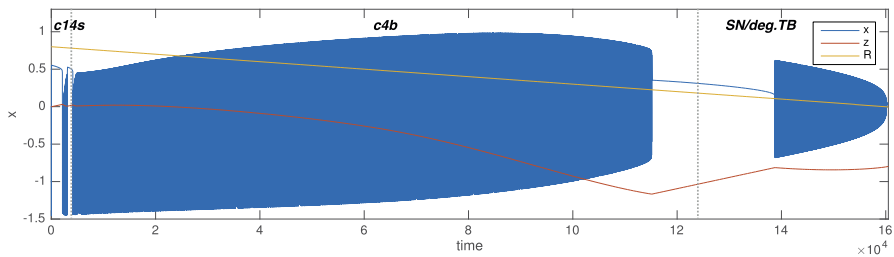
Fig. 18 Transitions across spheres. This timeseries is an example of transitions among classes due to a linear ultra-slow modulation of the radius R (in yellow). The \theta, \phi coordinates of A and B were kept constant and had the same values used to simulate c14s (at stage D). The next burst starts through SN_r and it ends (around R = 0.22 ) through FLC. The third burst starts again on SN_r and the oscillations stop at R = 0 when the fast subsystem undergoes the codim-3 deg. TB bifurcation
