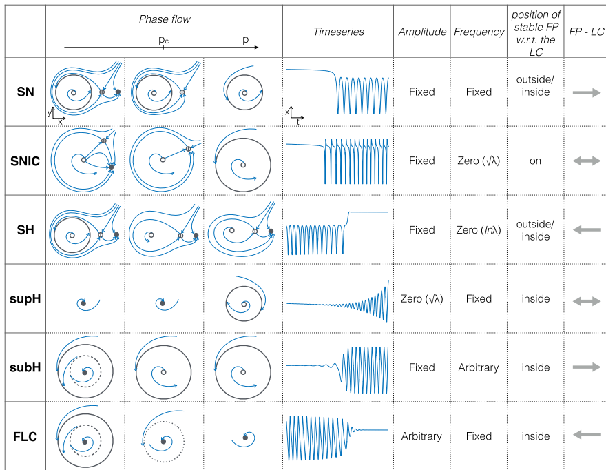
Fig. 2 Six planar bifurcations are responsible for oscillation onset and offset. In a dynamical system, a bifurcation occurs when a smooth change of the values of some of the parameters of the system causes a sudden qualitative change of its behavior. The parameters that need to be varied to have this change in behavior are called bifurcation parameters. The number of bifurcation parameters necessary gives the codimension of the bifurcation. In planar systems, only six types of codim-1 bifurcations can cause the transition from silent (stable fixed point, FP) to oscillatory (limit cycle, LC) behavior and/or vice versa. Their characteristics are illustrated in this figure. For each bifurcation we report an example of how the state space changes when varying the bifurcation parameter p . Bifurcations occur at the critical value p_c . Stable, saddle, unstable fixed points are represented by full , empty with a line inside , empty gray dots , respectively. Stable, half-stable, unstable limit cycles are shown with solid , dotted , dashed lines , respectively. Orbits appear in blue . We also show an example of timeseries and report the amplitude–frequency behavior, where \lambda = p - p_c . In the second last column we state whether the stable fixed point is inside or outside the stable limit cycle. This can affect the behavior of the baseline in the timeseries. The last column indicates the reversibility of the bifurcation, in the direction of the FP to the LC
