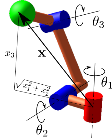
Figure 2: An example of orthogonal 3R serial robot
