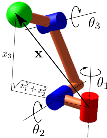
Figure 2: An example of orthogonal 3R serial robot
