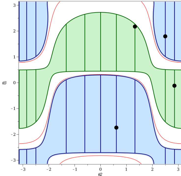
Figure 4: The angles that are associated to the projection on the plane associated to (c_2, s_2, c_3, s_3) of the sets under consideration. The sets S^+, S^- are represented as the areas in respectively green and blue while the red line represents the set V(\Delta) . Besides the black dots are the four inverse images of one sample point of \mathcal{P} . Finally we represent the roadmap of the projection of S^+ \cup S^- , containing these points, as the union of the green and blue lines, which belong to respectively S^+ and S^- .
