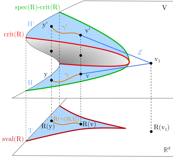
Figure 1: Illustration of the proof of Lemma 10.
