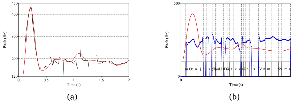
Figure 5: Raw f_0 (black) together with macromelodic (red) and micromelodic (blue) profiles for the first two seconds of recording A01
