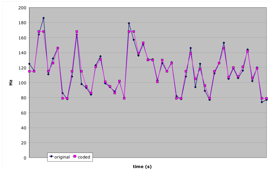
Figure 13: Predicted (pink) versus observed (blue) values for pitch anchor points for a 5 sentence passage after automatic coding with the INTSINT alphabet
