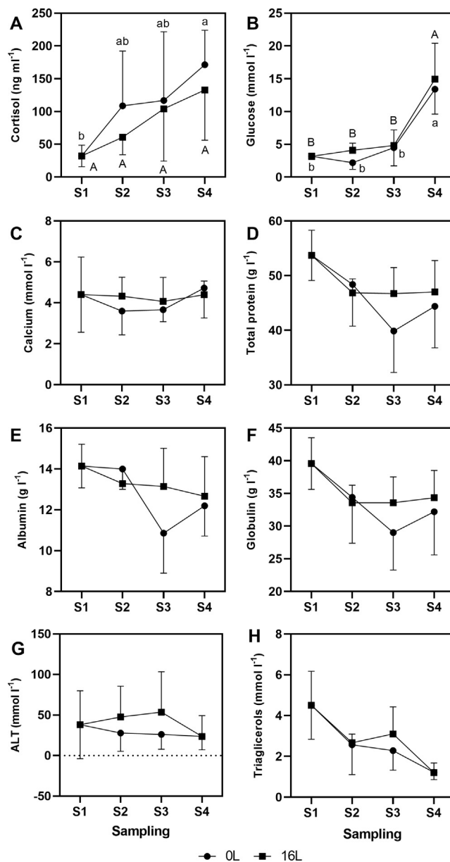
Fig. 5. Plasma cortisol levels and biochemical indices (mean ± SD) determined for female Eurasian perch throughout the course of the experiment, in which fish were exposed to either constant darkness (group OL) or a typical photoperiod (16 h light/8 h dark; group 16L), are shown. For an explanation of the sampling strategy used, please refer to Fig. 1. Between group differences were not significantly significant ( P > 0.05 ). Statistically significant differences ( P < 0.05 ) among the same group but between different sampling points were indicated with either lowercase (for group OL) or CAPITAL (for group 16L) letters. The absence of a letter indicates a lack of statistically significant difference. Abbreviations: ALT = alanine aminotransferase.
