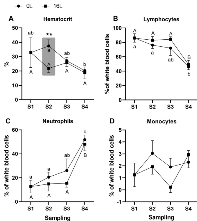
Fig. 4. Hematological indices (mean ± SD) were recorded for female Eurasian perch over the course of the experiment in which fish were exposed to either constant darkness (group OL) or a typical photoperiod (16 h light:8 h dark; group 16L). For an explanation of the sampling strategy used, please refer to Fig. 1. Statistical differences between groups are indicated using shadowed grey boxes marked with double asterisks ( P < 0.01 ). Statistically significant differences ( P < 0.05 ) among the same group but between different sampling points were indicated with either lowercase (for group OL) or CAPITAL (for group 16L) letters. The absence of a letter indicates a lack of statistically significant differences.
