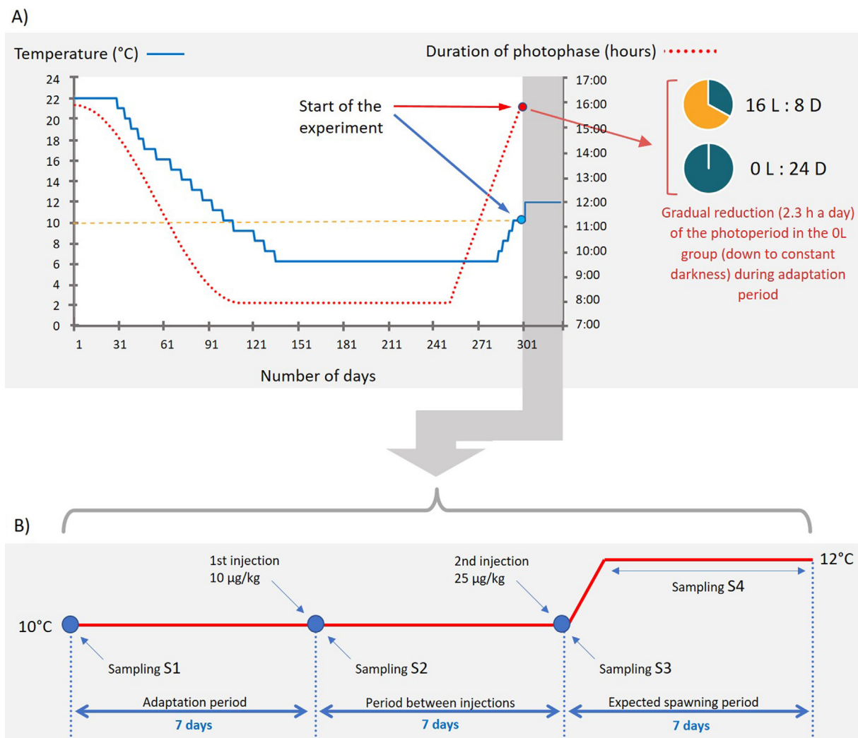
Fig. 1. A scheme summarising the overall experimental approach is shown. (A) The photo-thermal programme applied before initiation of the experiment (during which the fish in both groups were kept together and exposed for 301 days to the same photo-thermal conditions). (B) The thermal regime, experimental protocol (including hormonal treatment protocol) and sampling strategy used. 16L:8D refers to a group exposed to 16 h of light and 8 h of darkness per day. 0L:24D refers to group exposed to constant darkness.
