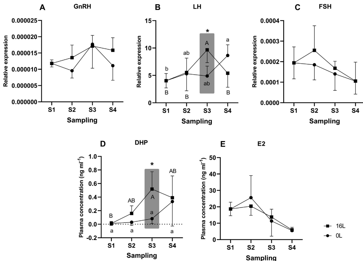
Fig. 3. Expression level of genes encoding gonadoliberin (GnRH), luteinising-hormone (LH), and follicle-stimulating-hormone (FSH), as well as blood plasma levels of DHP (17 \alpha , 20 \beta -dihydroxy-4-pregnen-3-one) and estradiol (E2) (mean \pm SD) in female Eurasian perch over the course of the experiment are shown. Fish were exposed to either constant darkness (group 0L) or a typical photoperiod (16 h light:8 h dark; group 16L). For an explanation of the sampling strategy, please refer to Fig. 1. Data determined for groups that are shadowed with a grey box and marked with an asterisk were determined to be different ( P < 0.05 ). Statistically significant differences ( P < 0.05 ) among the same group but between different sampling points were indicated with either lowercase (for group 0L) or CAPITAL (for group 16L) letters. The absence of a letter indicates a lack of statistically significant differences.
