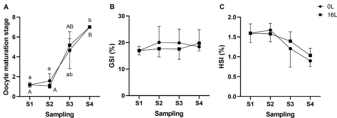
Fig. 2. Oocyte maturation stages, hepatosomatic (HSI), and gonadosomatic (GSI) indices (mean \pm SD) recorded in female Eurasian perch throughout the experimental period, in which fish were either exposed to constant darkness (group 0L) or a typically used photoperiod (16 h light:8 h dark; group 16L). For an explanation of the sampling strategy, please refer to Fig. 1. Data of both groups at each sampling point were not significantly different. The absence of a letter indicates a lack of statistically significant differences. Statistically significant differences ( P < 0.05 ) among the same group but between different sampling points were indicated with either lowercase (for group 0L) or CAPITAL (for group 16L) letters.
