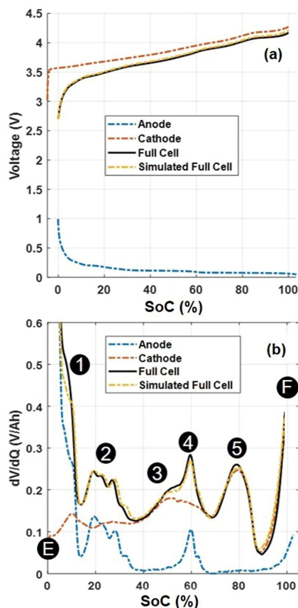
Figure 8. a) Voltage profiles obtained upon constant current charge at C/25 , 25^{\circ}\text{C} and b) differentiated voltage curves with respect to the capacity, versus SoC.
