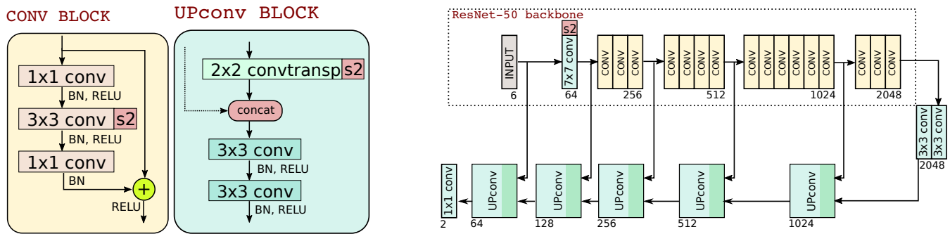
Figure 1. ResNet50-UNET architecture ( s2 = \text{stride } 2\text{px} ). The FC layer of ResNet50 has been removed. Numbers show output channels of each block.
