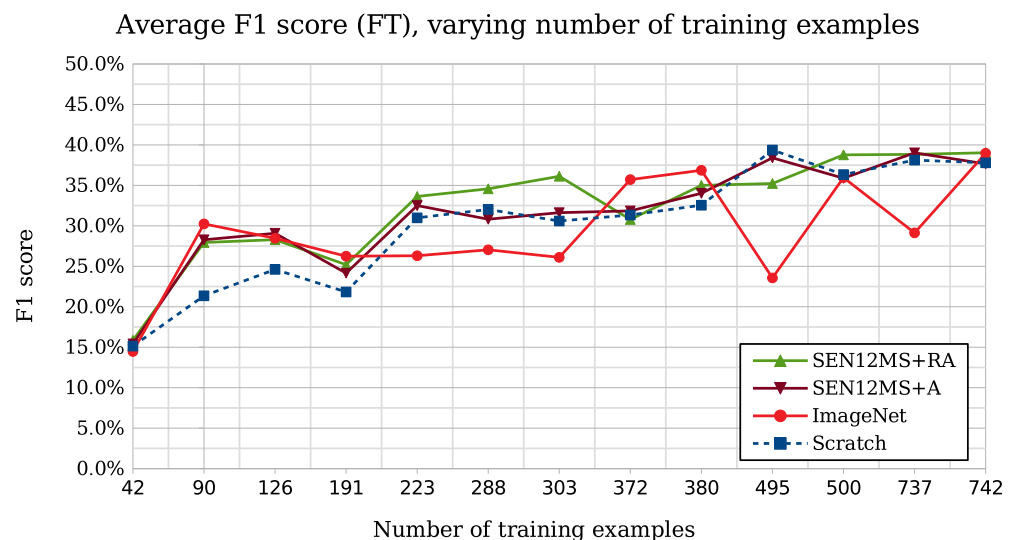
Figure 9. Impact of the number of training ships variation on mean F1 score calculated on Brest, Rotterdam, and Suez canal.
