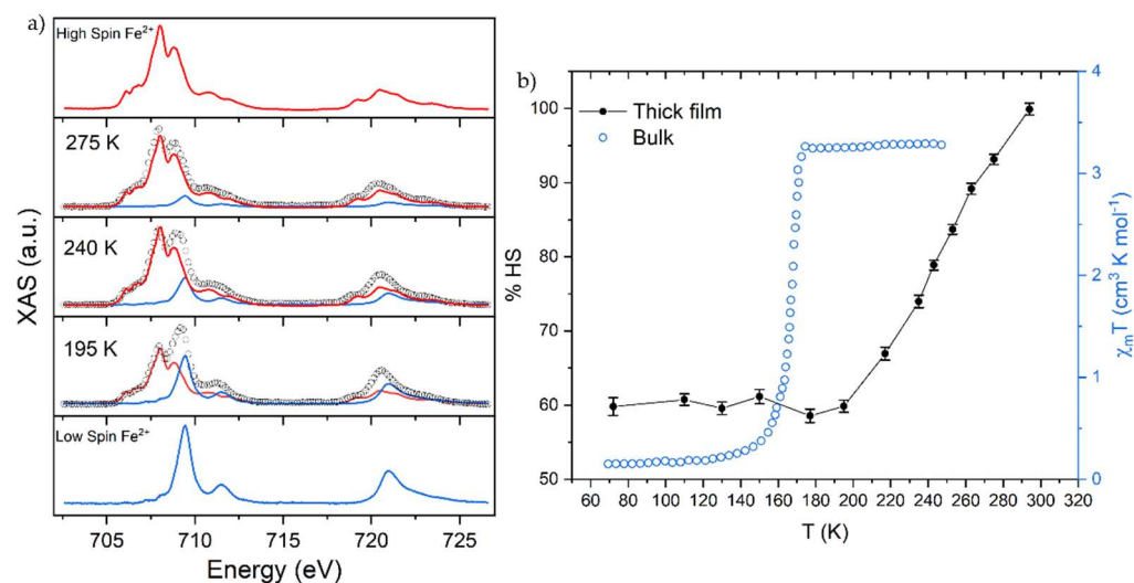
Figure 2. (a) Temperature dependence of normalized, experimental Fe L_{2,3} edge XAS spectra of [\text{Fe}(\text{H}_2\text{Bpz}_2)_2(\text{L})] thick film (empty dots) with contribution of high-spin \text{Fe}^{2+} (red line) and low-spin \text{Fe}^{2+} (blue line). [\text{Fe}(\text{H}_2\text{B}(\text{pz})_2)_2(2,2'\text{-bipy})] XAS spectra are taken as HS and LS references. Reprinted from Ref. [37]. (b) High-spin \text{Fe}^{2+} percentage distribution as a function of temperature (black dots) and magnetic susceptibility characterization of powder of [\text{Fe}(\text{H}_2\text{Bpz}_2)_2(\text{L})] . Reprinted from Ref. [21].
