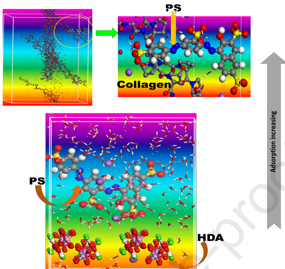
Fig. 12. Most stable configurations of two interfaces: PS/100water/50H 3 O + /50Cl - /Collagen and PS/100water/50H 3 O + /50Cl - /HDA at temperature of 297.15 K.
