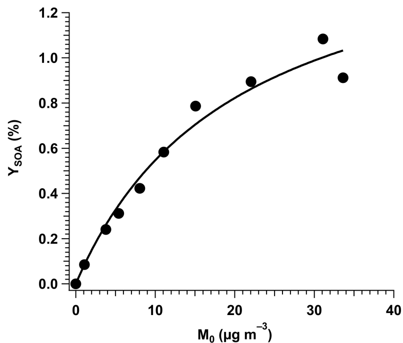
Figure 9. SOA formation yields Y_{\text{SOA}} vs. aerosol mass concentrations M_0 for T2P ozonolysis in the ASC chamber ( [\text{T2P}]_0 = 2.1 – 4.5 ppm and [\text{O}_3]_0 = 65 – 516 ppb). The line corresponds to a fit using Equation 8.
