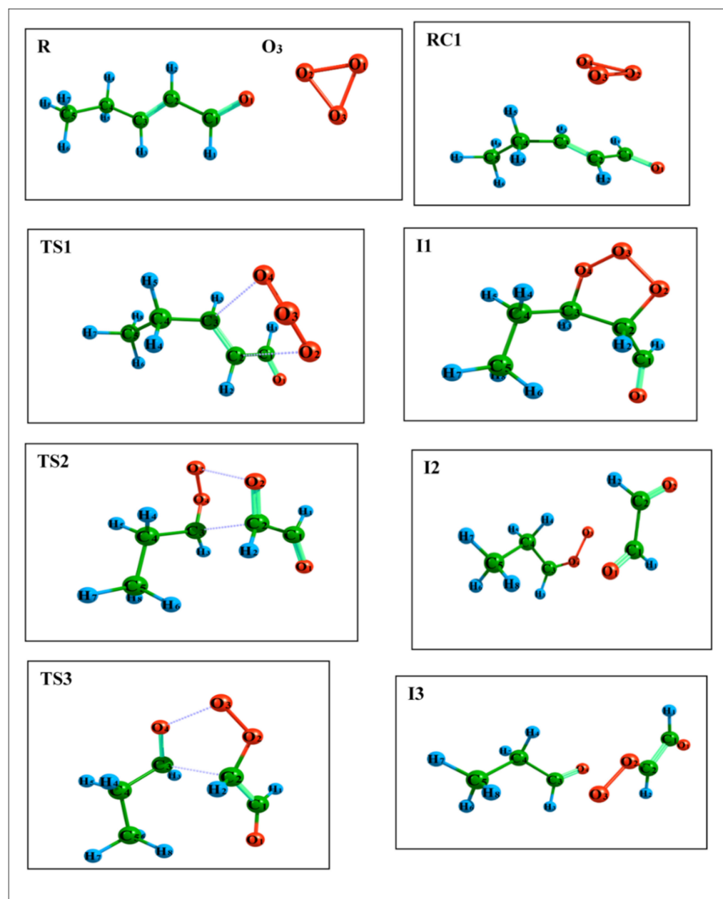
Figure 5. The optimized stationary points of the reaction of trans-2-pentenal with \text{O}_3 .
