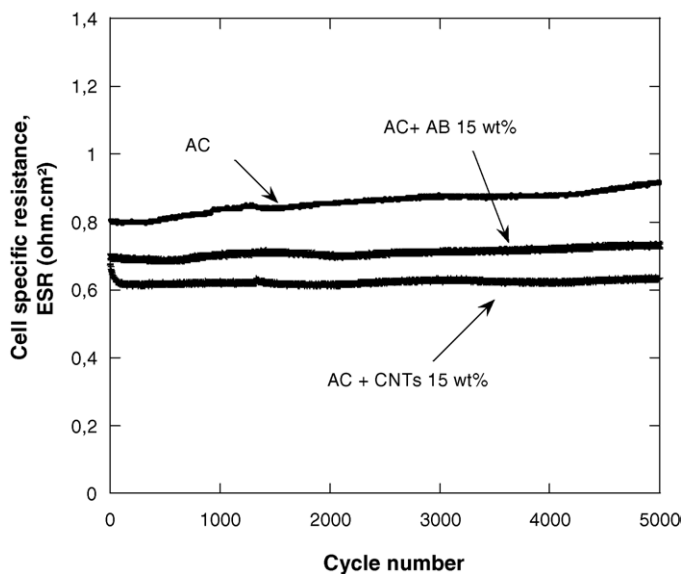
Fig. 5. ESR change during cycling between 0 and 2.3 V at \pm 25 \text{ mA/cm}^2 for the 4 \text{ cm}^2 supercapacitor cells assembled with the different active material compositions. Active material weight: 60 mg per electrode; electrolyte \text{NEt}_4\text{BF}_4 1.5 M in acetonitrile.
