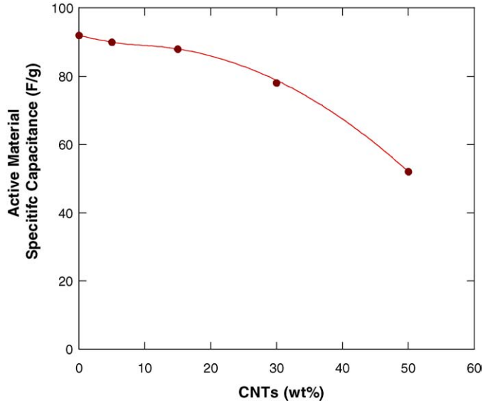
Fig. 3. Active material specific capacitance change vs. the MWCNTs content during galvanostatic cycling between 0 and 2.3 V; active material weight: 60 mg per electrode; electrolyte: \text{NEt}_4\text{BF}_4 1.5 M in acetonitrile.
