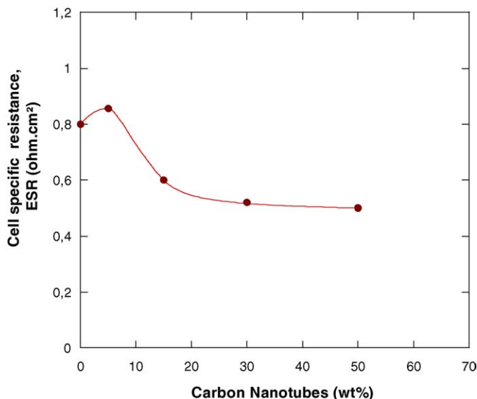
Fig. 2. ESR change of the cells vs. the active material MWCNTs content, up to 50 wt.%; active material weight: 60 mg per electrode; electrolyte \text{NEt}_4\text{BF}_4 1.5 M in acetonitrile.
