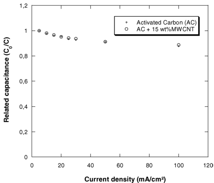
Fig. 4. Active material related capacitance ( C/C_0 ) change vs. the supercapacitor cell current density.
