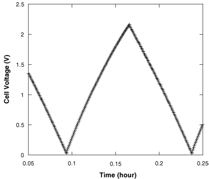
Fig. 1. Example of a charge/discharge plot at constant current ( 10 \text{ mA/cm}^2 ) obtained for the different supercapacitor cells; active material weight: 60 mg per electrode; electrolyte NEt 4 BF 4 1.5 M in acetonitrile.
