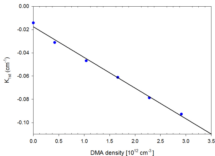
Fig. 12: Plot of the k_{1st} = -\beta [\text{DMA}] v as a function of the different DMA densities. The slope ( \beta / v ) of this plot multiplied by plasma velocity ( v = 1.85 \times 10^4 cm/s) gives us the electron attachment rate. In this example ( \beta = 4.8 \times 10^{-10} cm 3 s -1 ).
