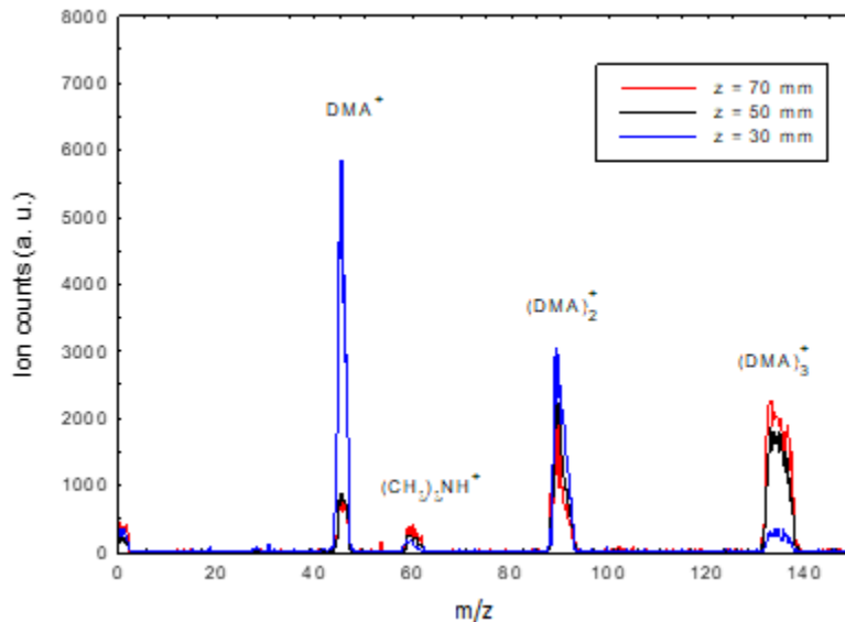
Fig. 7: Mass spectrum in the reaction chamber for a dimethylamine density of 4.5 \times 10^{12} \text{ cm}^{-3} taken at different z positions downstream from the injection port of the DMA/He mixture into an \text{Ar}^+ dominated plasma.
