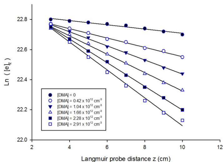
Fig. 11: Plots of the logarithm of different electron densities for different DMA concentrations as a function of different z positions along Langmuir probe distance.
