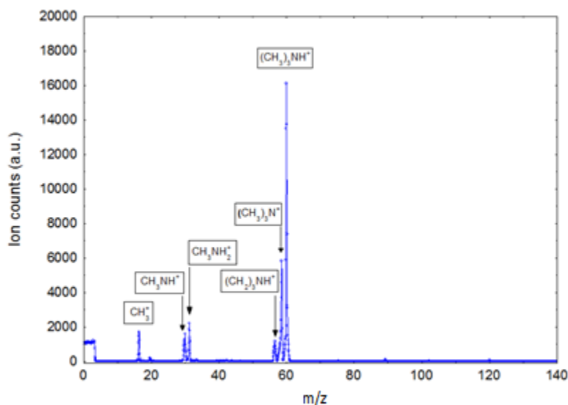
Fig. 2: Mass spectrum in the reaction chamber for a trimethylamine density of 1.4 \times 10^{12} \text{ cm}^{-3} taken at 30 mm downstream from the injection port of the TMA/He mixture into an \text{Ar}^+ dominated plasma.
