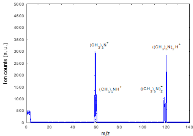
Fig. 3: Mass spectrum in the reaction chamber for a trimethylamine density of 4.0 \times 10^{12} \text{ cm}^{-3} taken at 30 mm downstream from the injection port of the TMA/He mixture into an \text{Ar}^+ dominated plasma.
