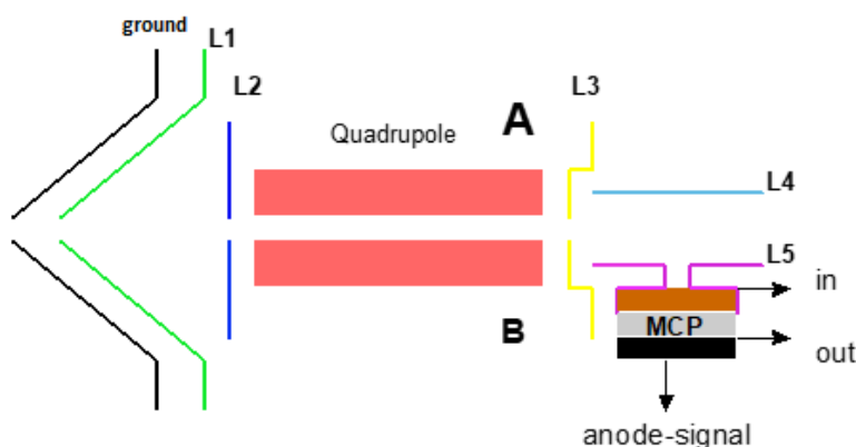
Fig. 13: Schematic of the lens structure of the quadrupole mass analyser in the FALP-MS apparatus.
