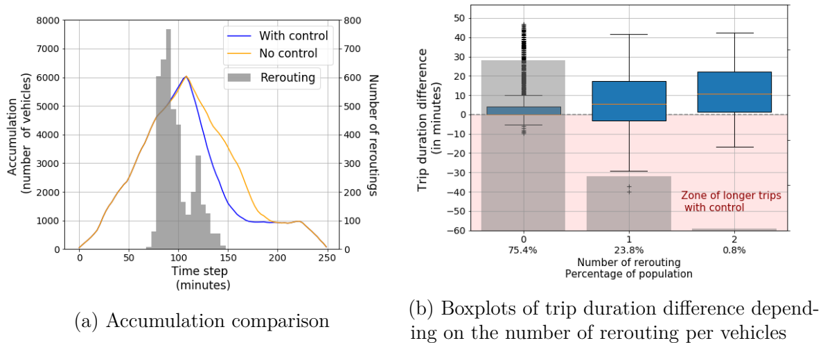
FIG. 1: Results on grid network of 5X5 areas
