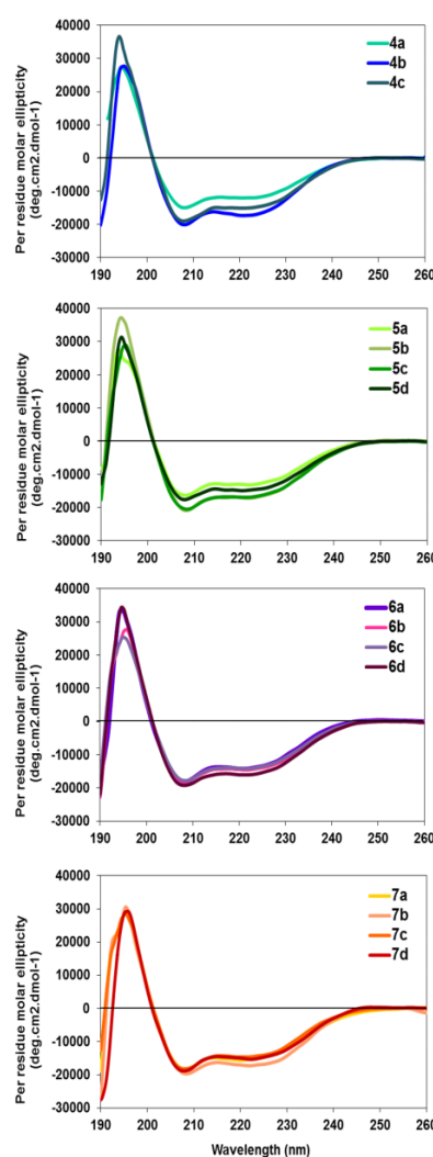
Figure 1. CD spectra of alamethicin F50/5 and its analogues (100µM) in methanol at 20°C.
