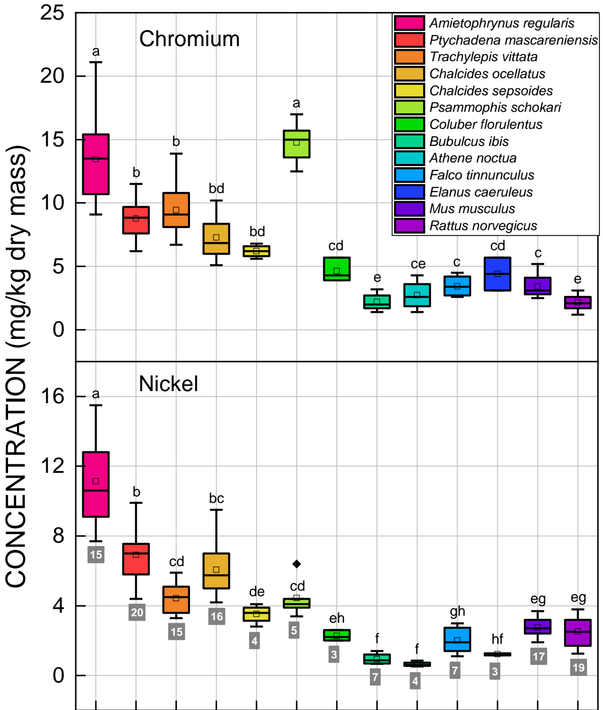
Figure 2. Mean metal concentrations in vertebrates from El-Tebbin area. Data are presented as mean \pm SD in mg/kg dry mass. Boxes followed by different letters denote significant differences in metal concentrations (analysis of variance [ANOVA]; Bonferroni test; P < 0.05 ). The number below each box indicates the number of samples. Metal concentrations are presented as means across sites A to G. The detailed Ni and Cr concentrations, for each site and each species, are presented in Supplementary materials 3-4 and 7.
