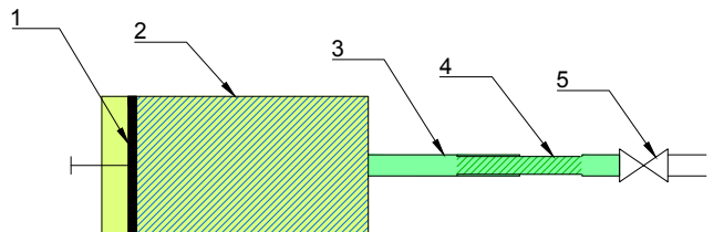
FIG. 4: Schematic drawing of the RLC resonator : (1) Sealed piston, (2) Variable capacitance, (3) Fixed inductance, (4) Variable inductance, (5) Micrometric needle valve.
