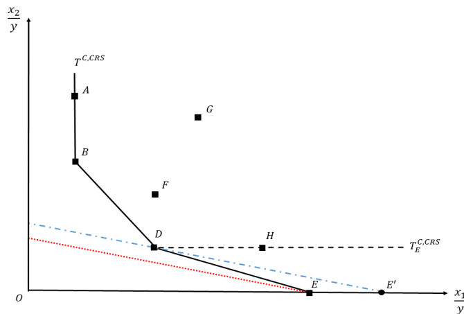
Figure 2: Isoquant with combinations of two inputs and single output under convexity and CRS assumptions
